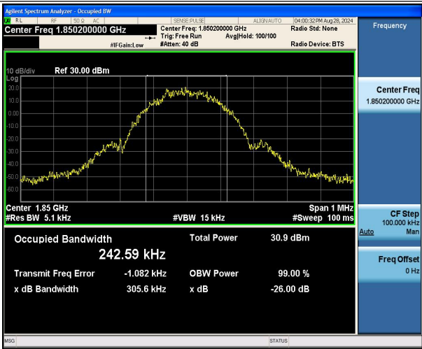
EGPRS1900-512-2-PASS
