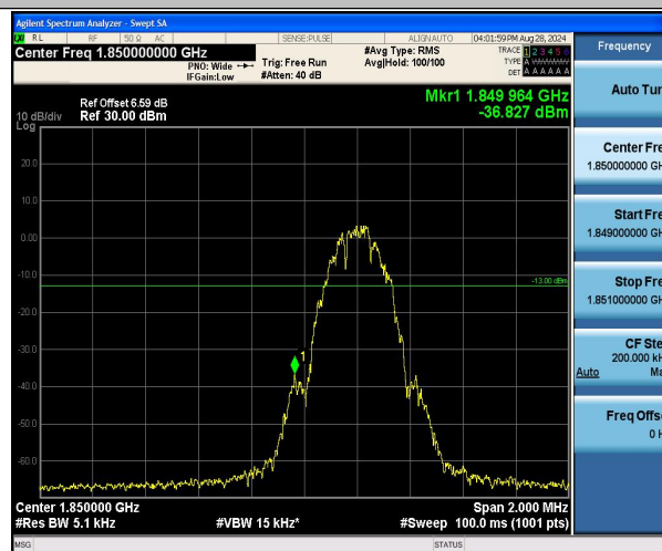
EGPRS1900-512-2-PASS
