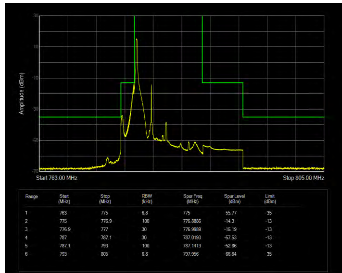
Band13 16QAM BW=5MHz Channel=23205 RB Size=1 Position=#Max Normal
