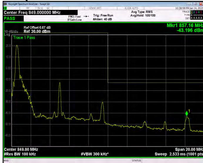
Band5 16QAM BW=10MHz Channel=20600 RB Size=1 Position=#Max Extended
