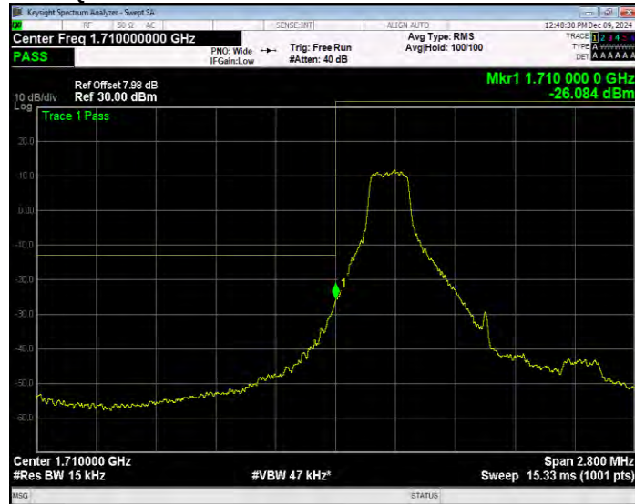
Band66 16QAM BW=1.4MHz Channel=131979 RB Size=1 Position=#Max Extended
