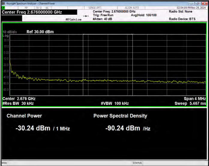
Band41(2535-2675) 16QAM BW=20MHz Channel=41340 RB Size=100 Position=#0 Normal
