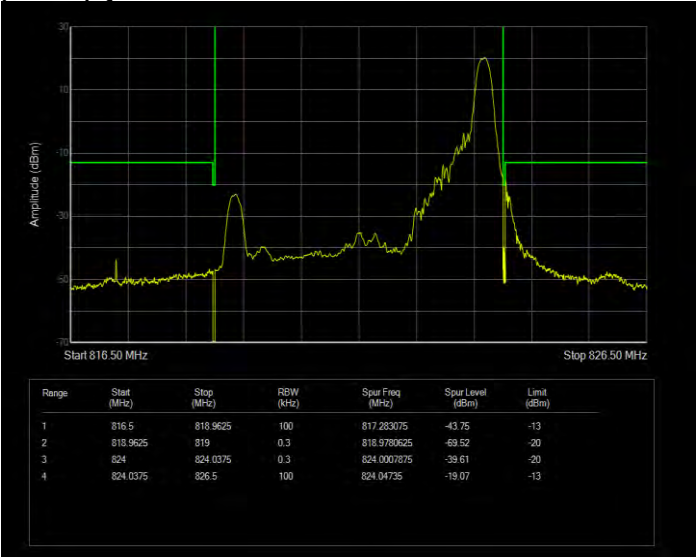
Band26(814-824) QPSK BW=5MHz Channel=26765 RB Size=25 Position=#0 Extended
