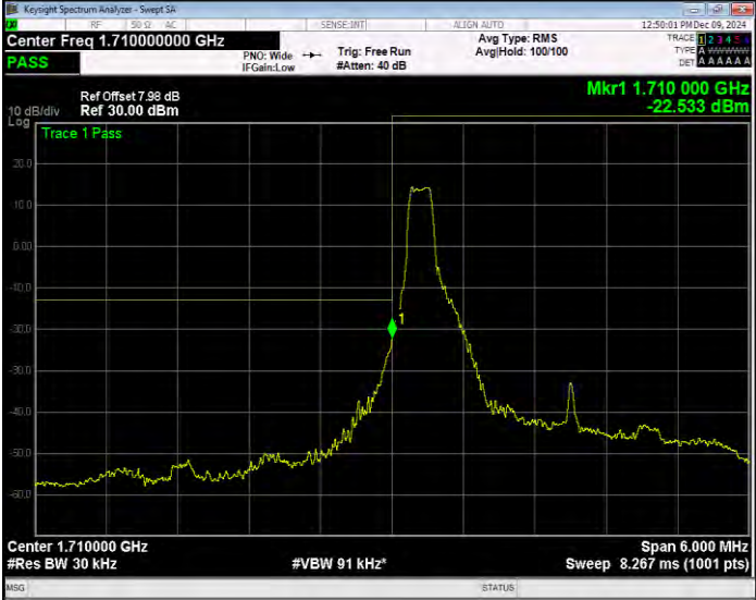
Band66 16QAM BW=3MHz Channel=131987 RB Size=1 Position=#Max Extended
