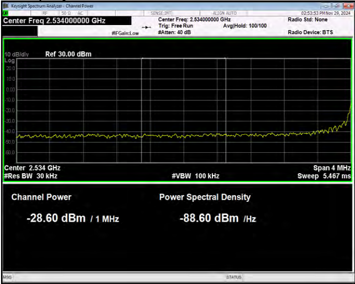
Band41(2535-2675) 16QAM BW=20MHz Channel=40140 RB Size=100 Position=#0 Extended
