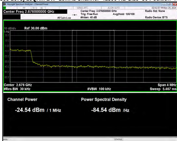
Band41(2535-2675) 16QAM BW=10MHz Channel=41390 RB Size=50 Position=#0 Extended
