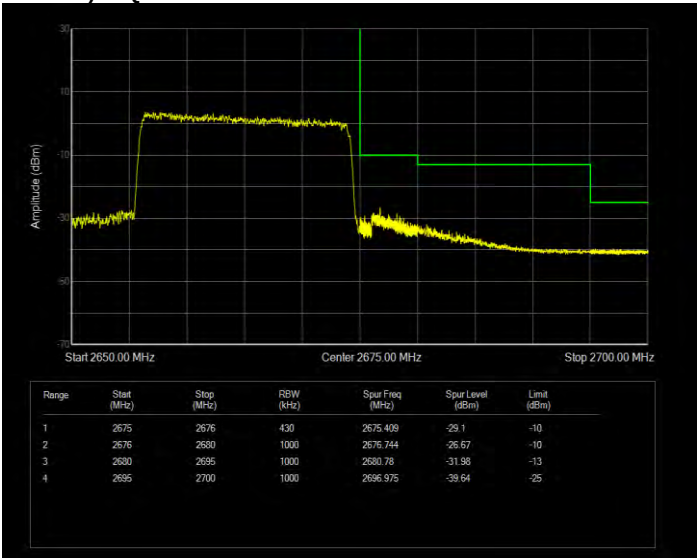
Band41(2535-2675) 16QAM BW=20MHz Channel=41340 RB Size=100 Position=#0 Normal
