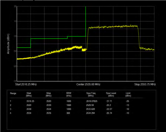
Band41(2535-2675) 16QAM BW=15MHz Channel=40115 RB Size=75 Position=#0 Normal
