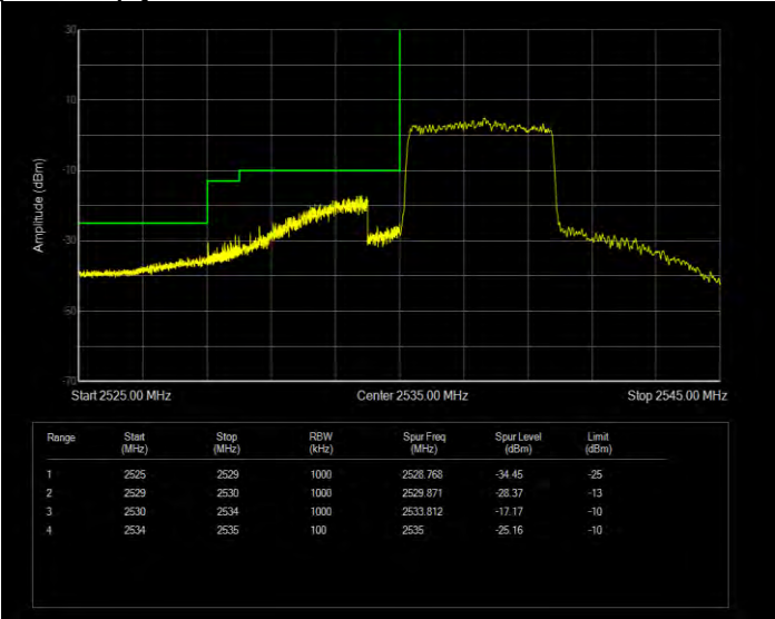
Band41(2535-2675) QPSK BW=5MHz Channel=40065 RB Size=25 Position=#0 Normal
