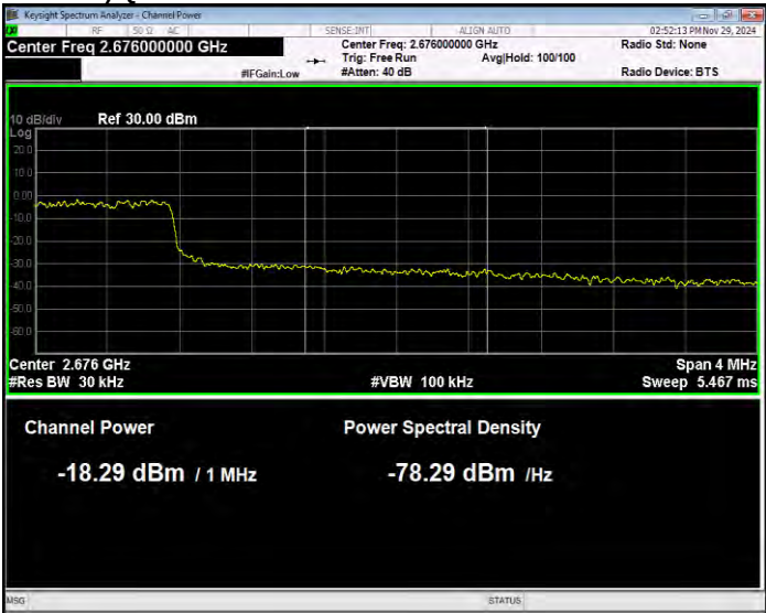
Band41(2535-2675) QPSK BW=5MHz Channel=41415 RB Size=25 Position=#0 Normal
