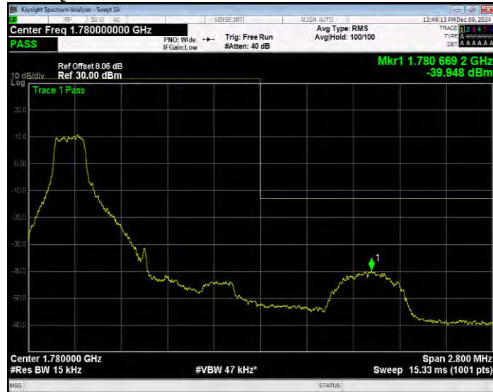
Band66 16QAM BW=1.4MHz Channel=132665 RB Size=1 Position=#Max Extended
