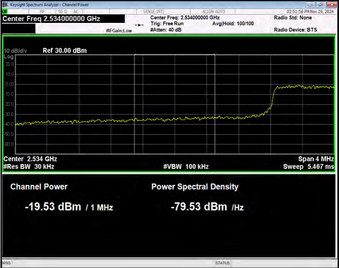
Band41(2535-2675) QPSK BW=5MHz Channel=40065 RB Size=25 Position=#0 Normal
