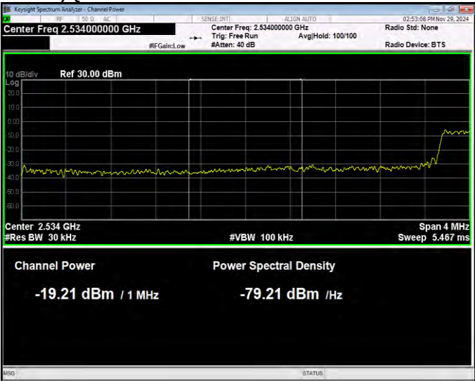
Band41(2535-2675) QPSK BW=15MHz Channel=40115 RB Size=75 Position=#0 Extended
