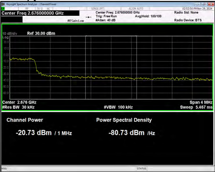
Band41(2535-2675) QPSK BW=10MHz Channel=41390 RB Size=50 Position=#0 Normal
