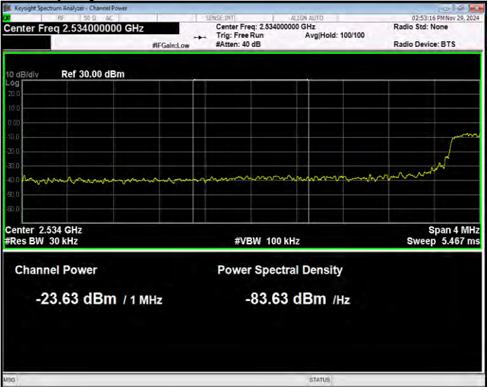
Band41(2535-2675) 16QAM BW=15MHz Channel=40115 RB Size=75 Position=#0 Normal
