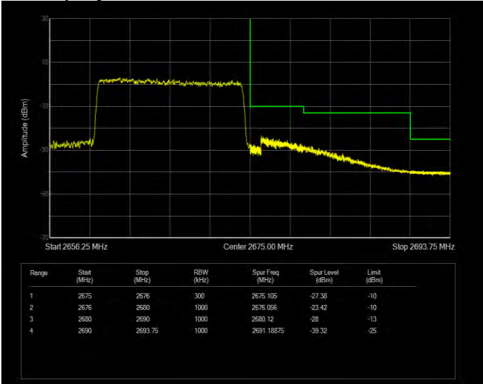
Band41(2535-2675) 16QAM BW=20MHz Channel=40140 RB Size=100 Position=#0 Extended
