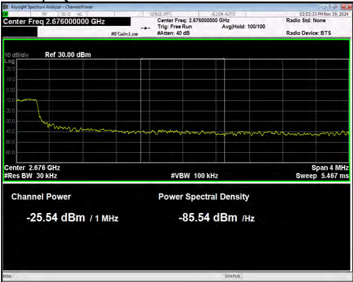
Band41(2535-2675) 16QAM BW=15MHz Channel=41365 RB Size=75 Position=#0 Normal
