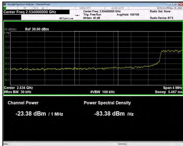
Band41(2535-2675) 16QAM BW=10MHz Channel=40090 RB Size=50 Position=#0 Normal
