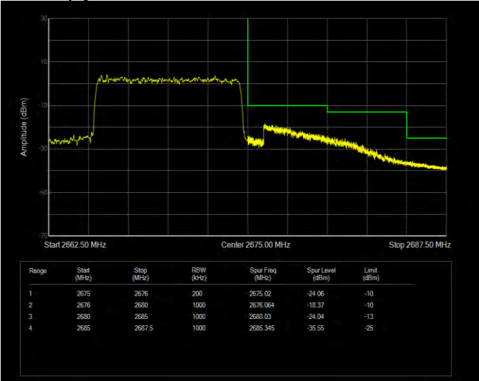
Band41(2535-2675) QPSK BW=15MHz Channel=40115 RB Size=75 Position=#0 Extended
