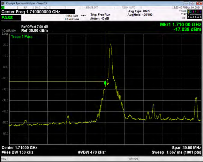
Band66 QPSK BW=15MHz Channel=132047 RB Size=1 Position=#Max Extended
