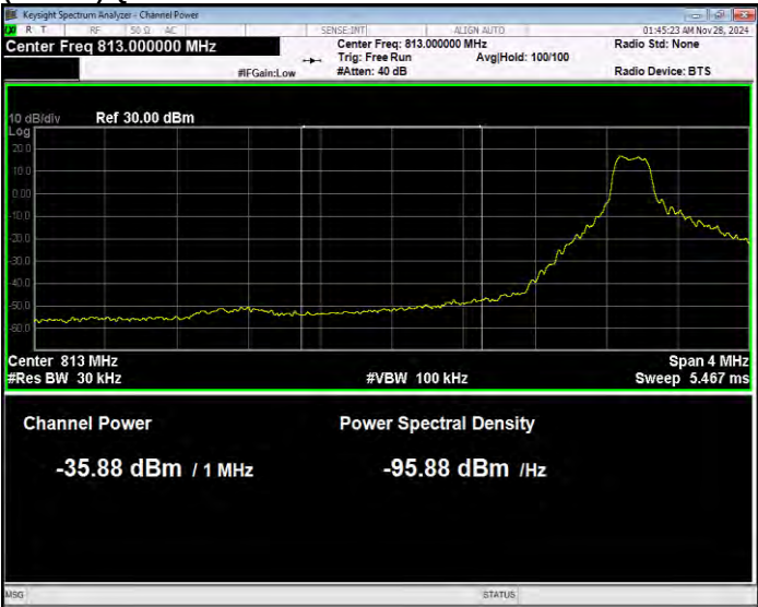
Band26(814-824) QPSK BW=5MHz Channel=26715 RB Size=1 Position=#0 Normal
