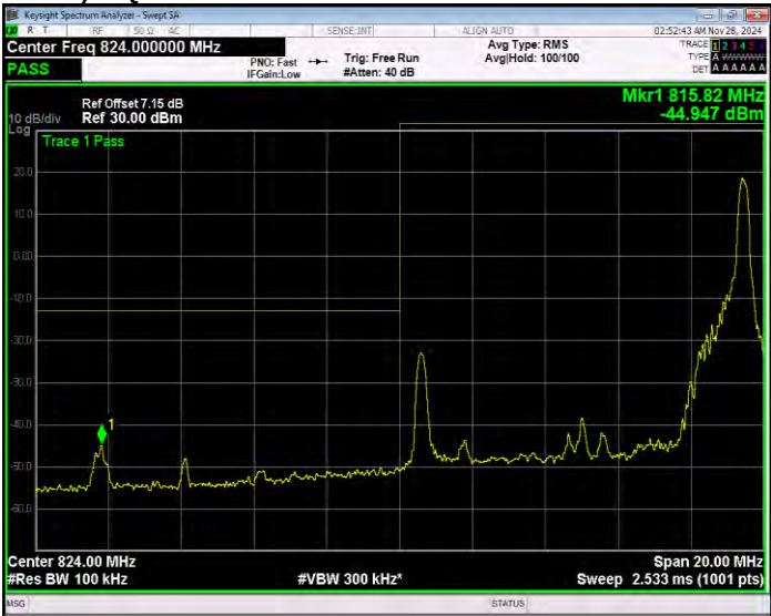
Band26(824-849) 16QAM BW=10MHz Channel=26840 RB Size=50 Position=#0 Extended
