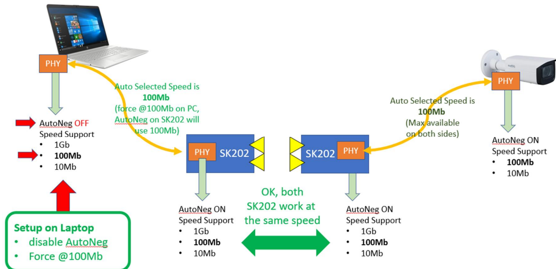
Figure 4. Controlled auto-negotiation is required when the 2 devices do not advertise the same maximum speed capability
