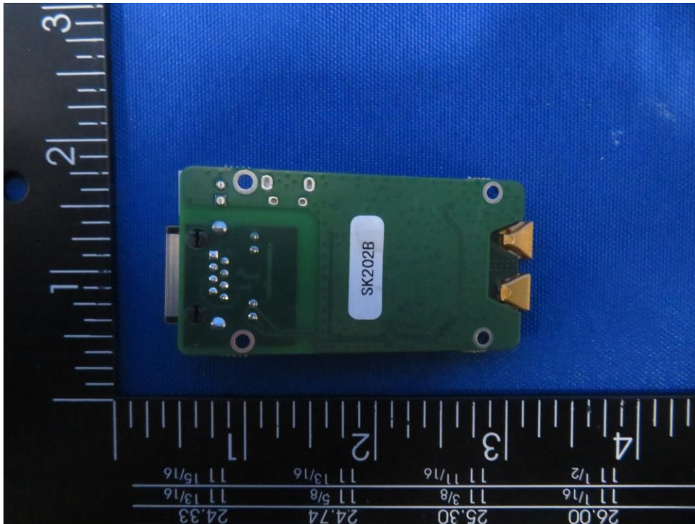
(3) EUT Photo – SK202B
