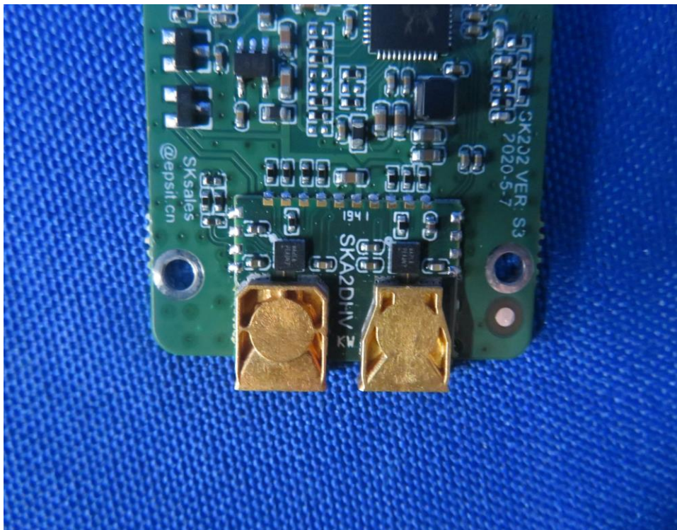
(2) EUT Photo – SK202A
