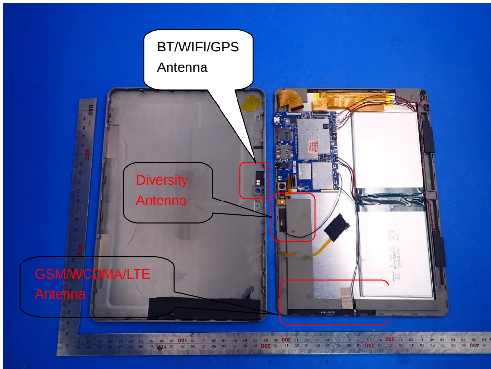
WIFI&BT&GPS ANTENNA
