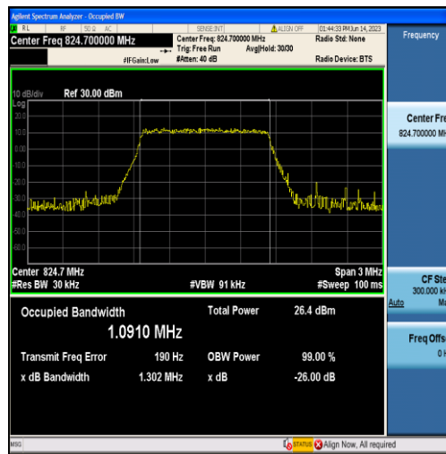
Band5-1.4MHz-QPSK-20407-6RB#0-1.0910
