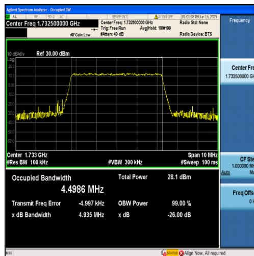
Band4-5MHz-QPSK-20175-25RB#0-4.4986
