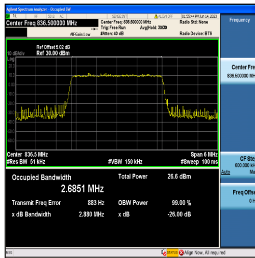
Band5-3MHz-16QAM-20525-15RB#0-2.6851
