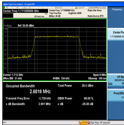
Band4-3MHz-16QAM-19965-15RB#0-2.6818
