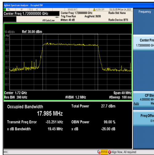
Band4-20MHz-16QAM-20050-100RB#0-17.985
