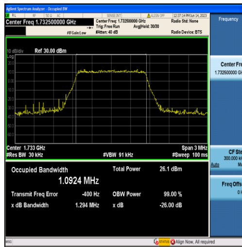
Band4-1.4MHz-16QAM-20175-6RB#0-1.0924
