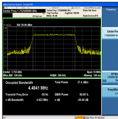
Band4-5MHz-16QAM-20375-25RB#0-4.4841
