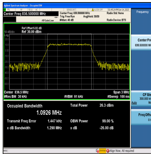
Band5-1.4MHz-16QAM-20525-6RB#0-1.0926
