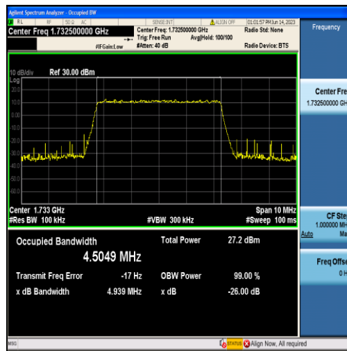
Band4-5MHz-16QAM-20175-25RB#0-4.5049
