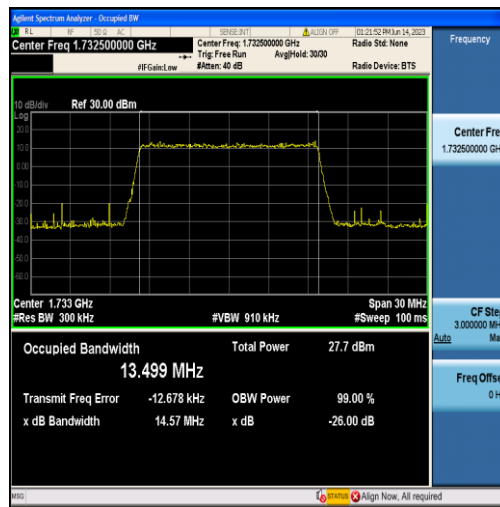
Band4-15MHz-16QAM-20175-75RB#0-13.499
