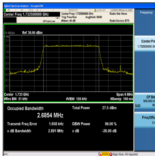
Band4-3MHz-QPSK-20175-15RB#0-2.6854
