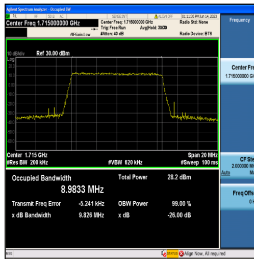
Band4-10MHz-QPSK-20000-50RB#0-8.9833
