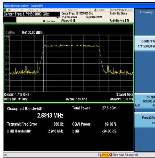
Band4-3MHz-QPSK-19965-15RB#0-2.6913
