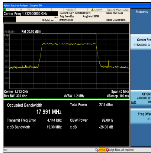
Band4-20MHz-16QAM-20175-100RB#0-17.991
