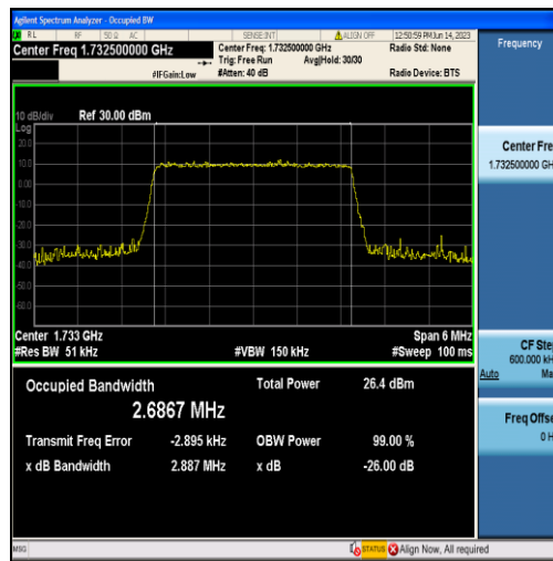
Band4-3MHz-16QAM-20175-15RB#0-2.6867
