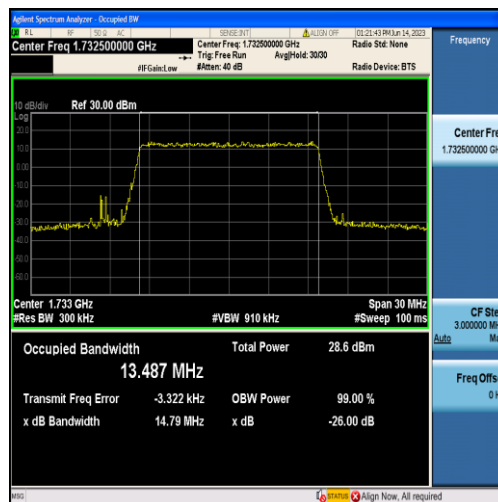
Band4-15MHz-QPSK-20175-75RB#0-13.487
