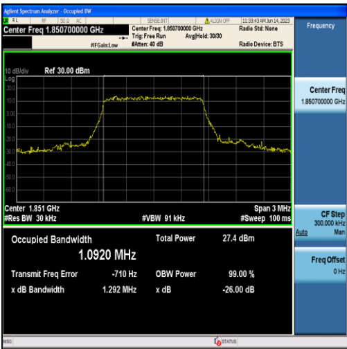
Band2-1.4MHz-QPSK-18607-6RB#0-1.0920
