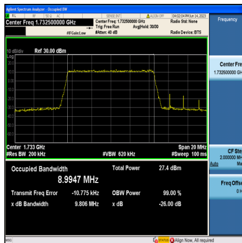
Band4-10MHz-16QAM-20175-50RB#0-8.9947
