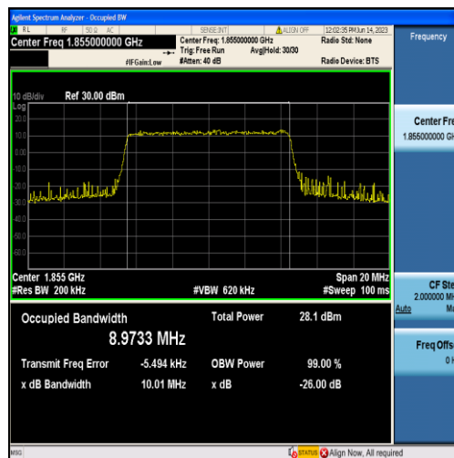
Band2-10MHz-16QAM-18650-50RB#0-8.9733
