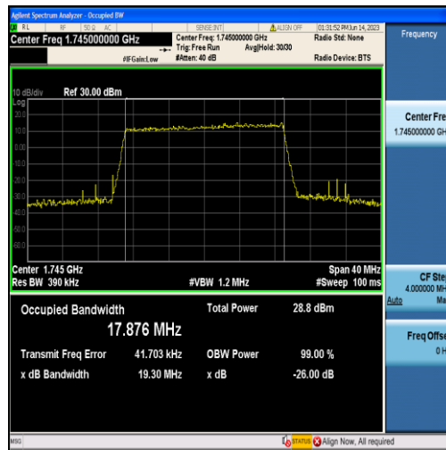
Band4-20MHz-QPSK-20300-100RB#0-17.876
