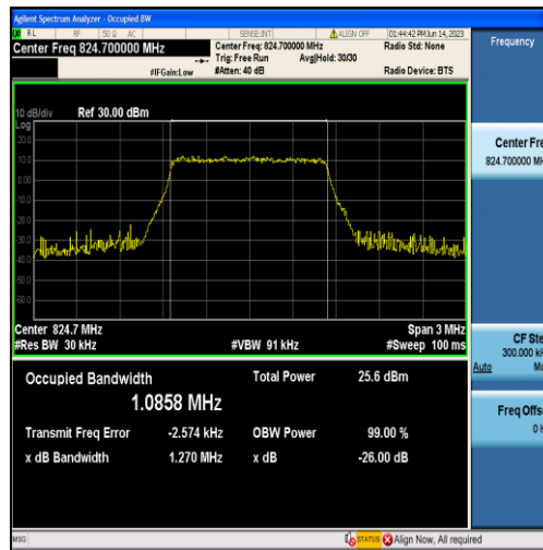
Band5-1.4MHz-16QAM-20407-6RB#0-1.0858
