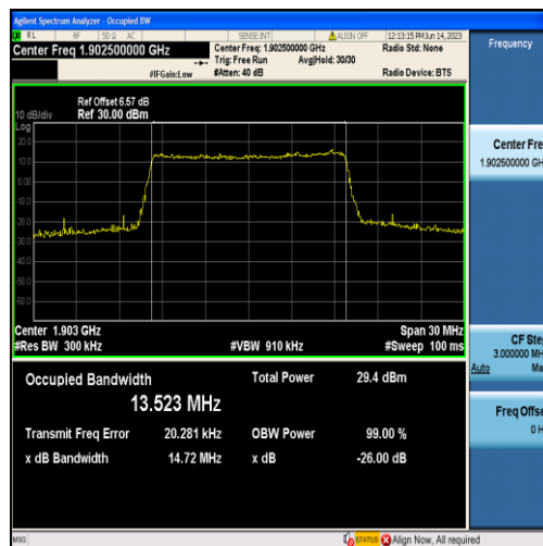
Band2-15MHz-QPSK-19125-75RB#0-13.523
