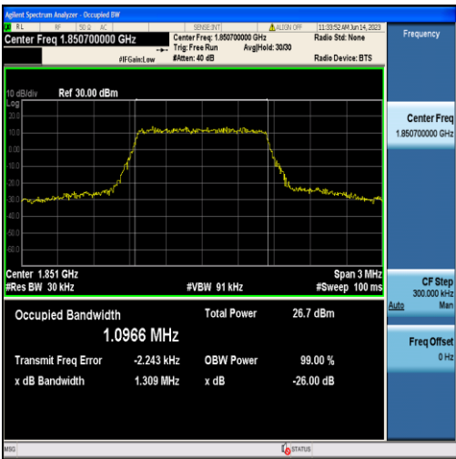
Band2-1.4MHz-16QAM-18607-6RB#0-1.0966
