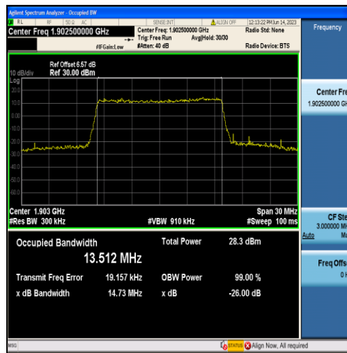
Band2-15MHz-16QAM-19125-75RB#0-13.512
