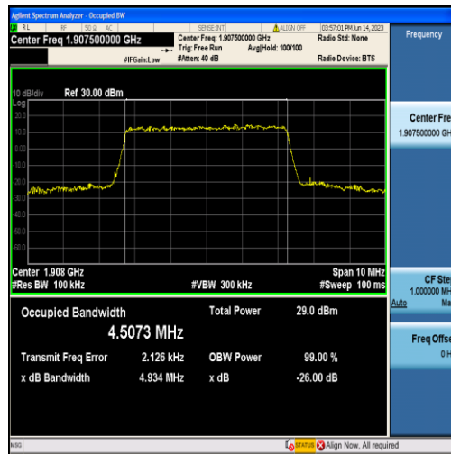
Band2-5MHz-QPSK-19175-25RB#0-4.5073
