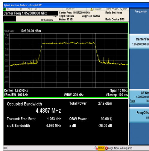
Band2-5MHz-16QAM-18625-25RB#0-4.4857
