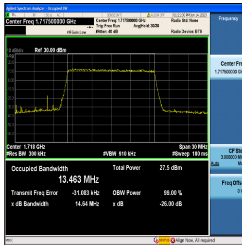
Band4-15MHz-16QAM-20025-75RB#0-13.463
