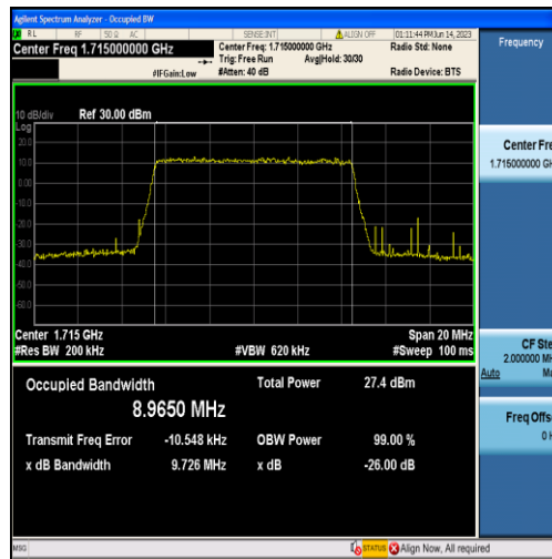
Band4-10MHz-16QAM-20000-50RB#0-8.9650
