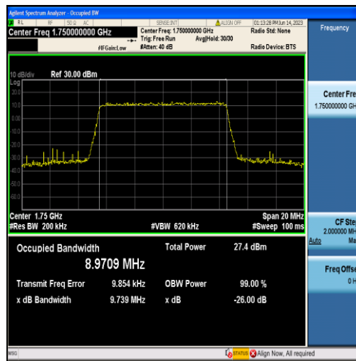
Band4-10MHz-16QAM-20350-50RB#0-8.9709
