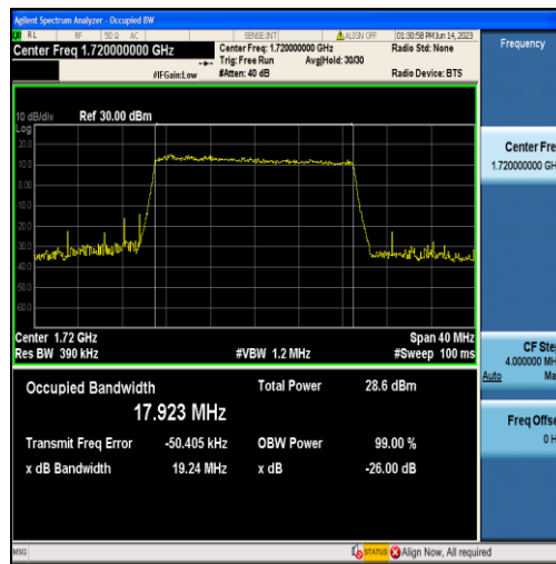
Band4-20MHz-QPSK-20050-100RB#0-17.923
