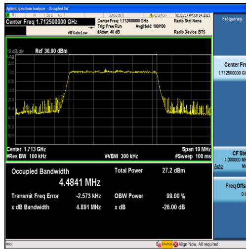
Band4-5MHz-16QAM-19975-25RB#0-4.4841
