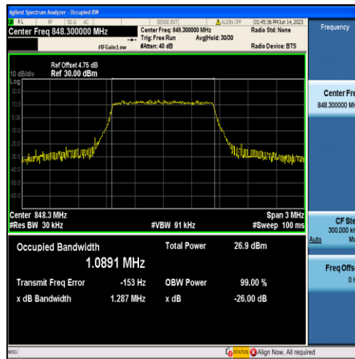
Band5-1.4MHz-QPSK-20643-6RB#0-1.0891
