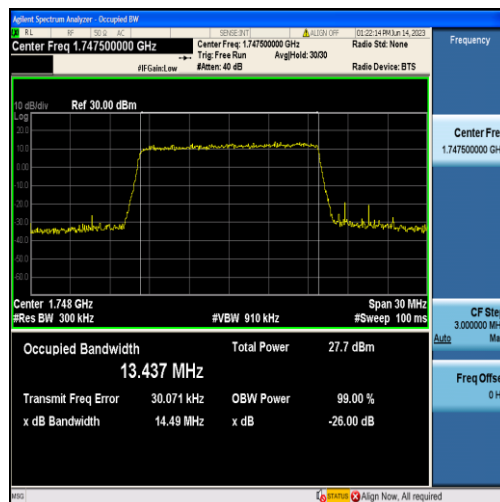
Band4-15MHz-16QAM-20325-75RB#0-13.437
