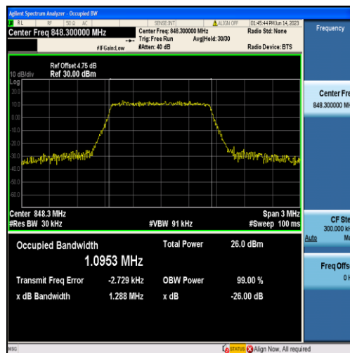
Band5-1.4MHz-16QAM-20643-6RB#0-1.0953
