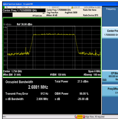
Band4-3MHz-QPSK-20385-15RB#0-2.6881
