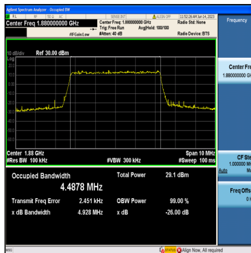
Band2-5MHz-QPSK-18900-25RB#0-4.4878
