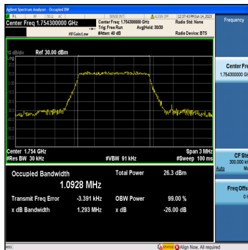
Band4-1.4MHz-16QAM-20393-6RB#0-1.0928
