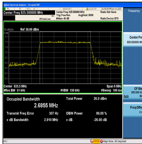
Band5-3MHz-16QAM-20415-15RB#0-2.6855
