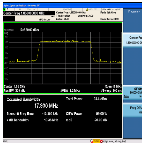
Band2-20MHz-16QAM-18700-100RB#0-17.930
