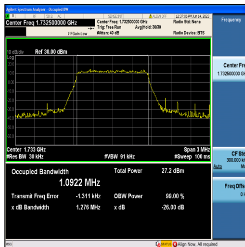
Band4-1.4MHz-QPSK-20175-6RB#0-1.0922
