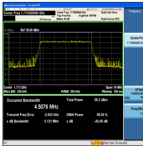
Band4-5MHz-QPSK-19975-25RB#0-4.5076
