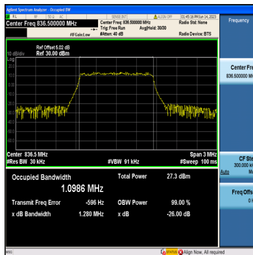
Band5-1.4MHz-QPSK-20525-6RB#0-1.0986
