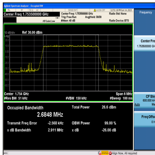
Band4-3MHz-16QAM-20385-15RB#0-2.6848
