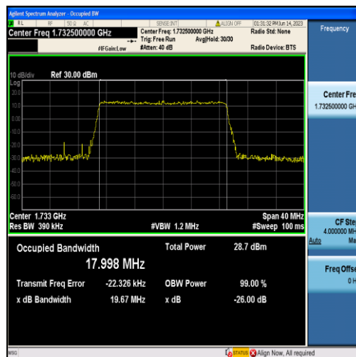
Band4-20MHz-QPSK-20175-100RB#0-17.998
