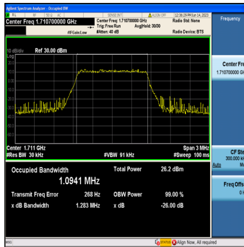
Band4-1.4MHz-16QAM-19957-6RB#0-1.0941
