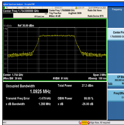
Band4-1.4MHz-QPSK-20393-6RB#0-1.0925
