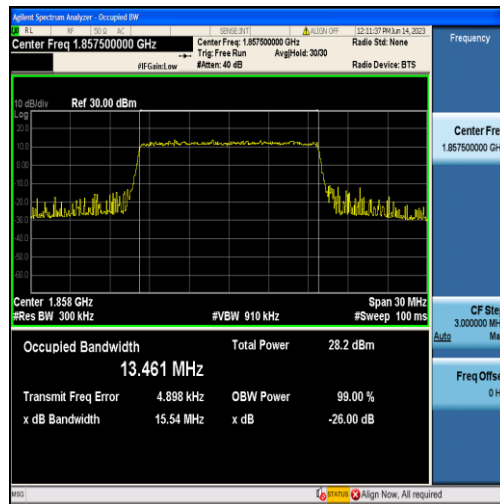
Band2-15MHz-16QAM-18675-75RB#0-13.461
