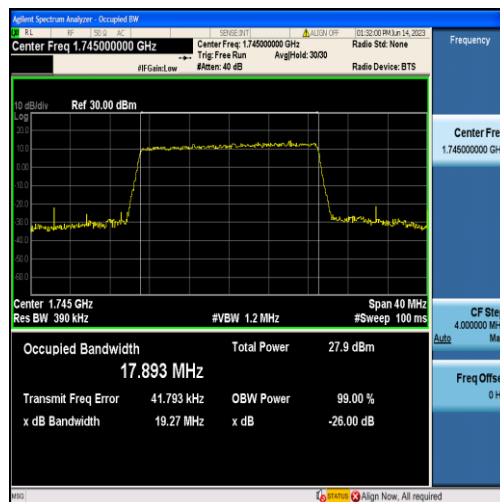
Band4-20MHz-16QAM-20300-100RB#0-17.893
