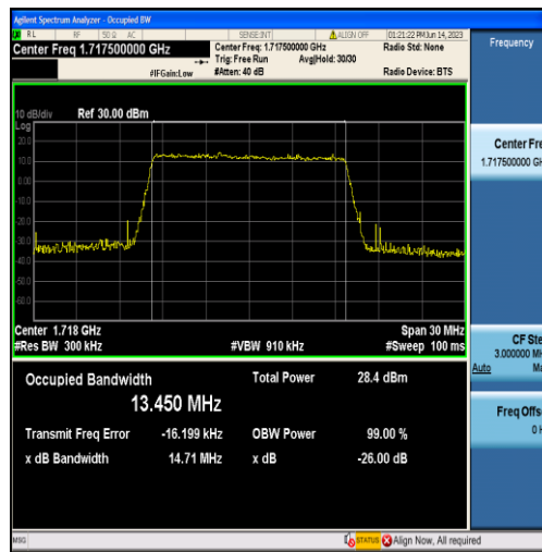
Band4-15MHz-QPSK-20025-75RB#0-13.450
