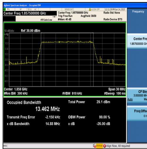
Band2-15MHz-QPSK-18675-75RB#0-13.462
