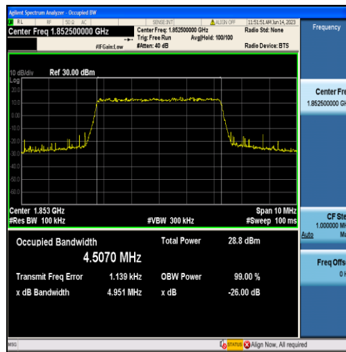
Band2-5MHz-QPSK-18625-25RB#0-4.5070
