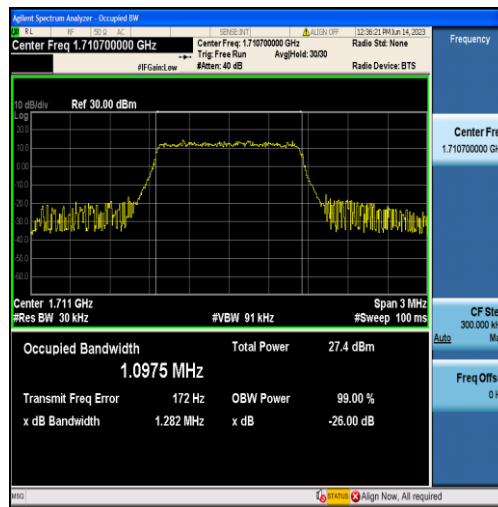
Band4-1.4MHz-QPSK-19957-6RB#0-1.0975
