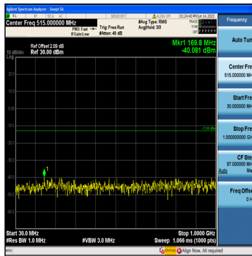
Band4-15MHz-16QAM-20325-75RB#0-Range1:30~1000MHz
