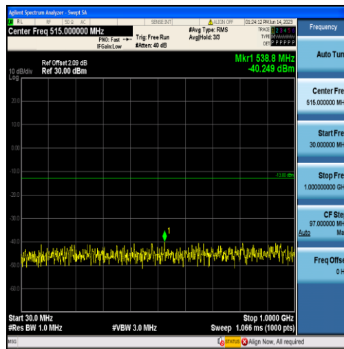
Band4-15MHz-QPSK-20175-75RB#0-Range1:30~1000MHz
