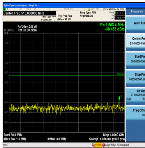
Band4-20MHz-16QAM-20300-100RB#0-Range1:30~1000MHz
