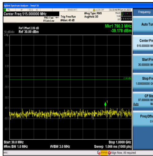
Band4-20MHz-QPSK-20175-100RB#0-Range1:30~1000MHz
