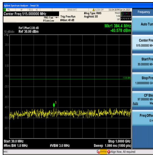
Band4-5MHz-16QAM-20375-25RB#0-Range1:30~1000MHz
