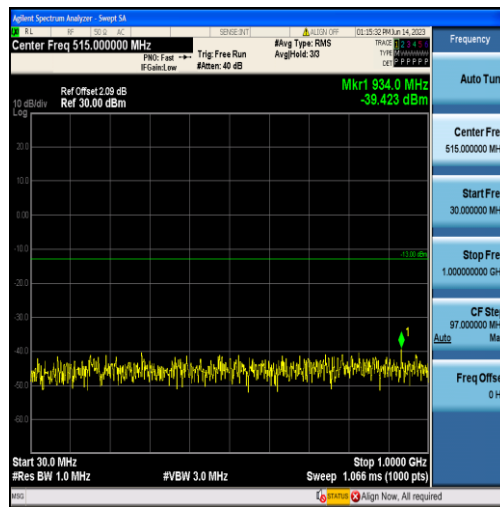
Band4-10MHz-16QAM-20350-50RB#0-Range1:30~1000MHz
