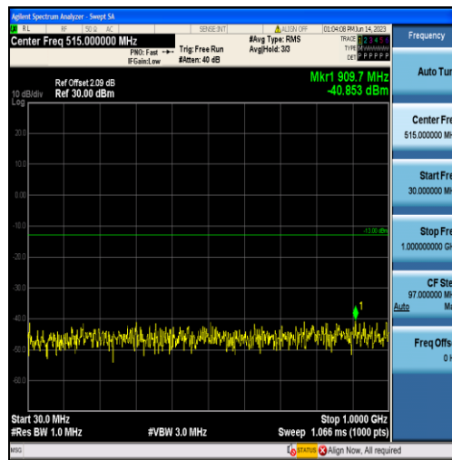
Band4-5MHz-QPSK-20175-25RB#0-Range1:30~1000MHz
