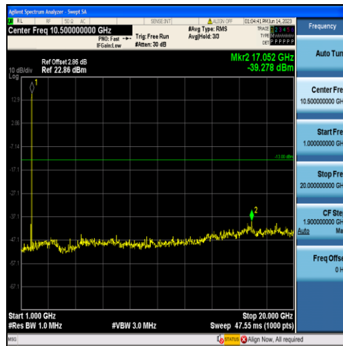
Band4-5MHz-16QAM-20375-25RB#0-Range2:1000~20000MHz
