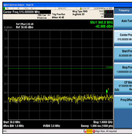
Band4-3MHz-QPSK-20175-15RB#0-Range1:30~1000MHz
