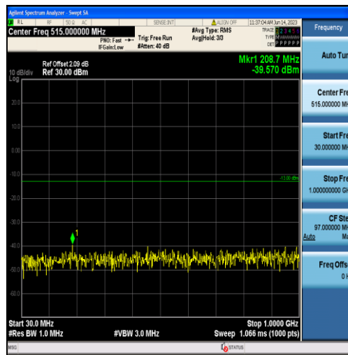
Band2-1.4MHz-16QAM-19193-6RB#0-Range1:30~1000MHz
