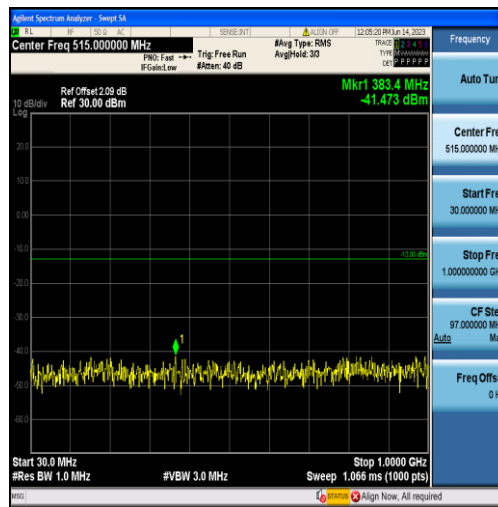
Band2-10MHz-QPSK-18900-50RB#0-Range1:30~1000MHz
