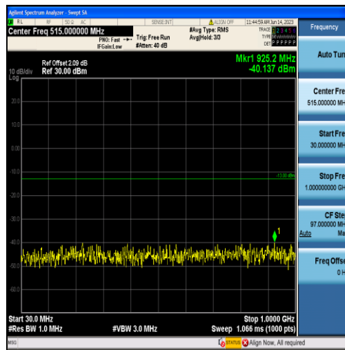
Band2-3MHz-QPSK-18900-15RB#0-Range1:30~1000MHz
