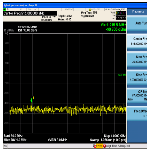
Band4-1.4MHz-QPSK-20175-6RB#0-Range1:30~1000MHz
