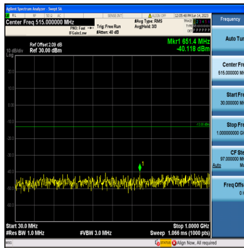
Band2-10MHz-16QAM-19150-50RB#0-Range1:30~1000MHz
