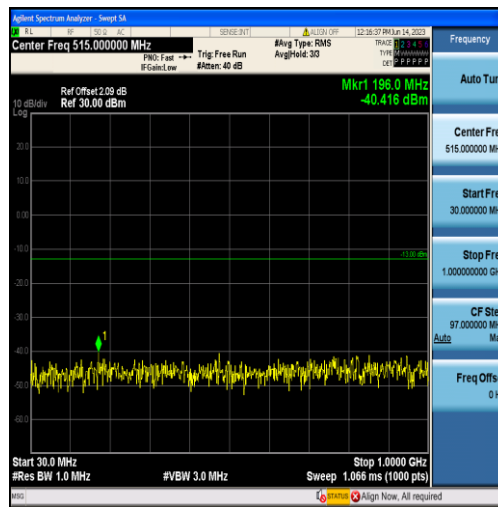
Band2-15MHz-16QAM-19125-75RB#0-Range1:30~1000MHz
