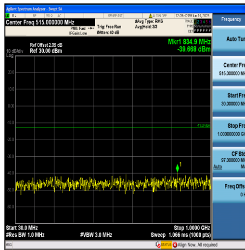
Band2-20MHz-16QAM-19100-100RB#0-Range1:30~1000MHz
