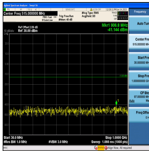
Band2-20MHz-QPSK-18900-100RB#0-Range1:30~1000MHz
