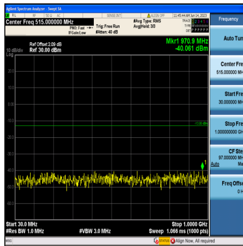
Band2-3MHz-16QAM-19185-15RB#0-Range1:30~1000MHz
