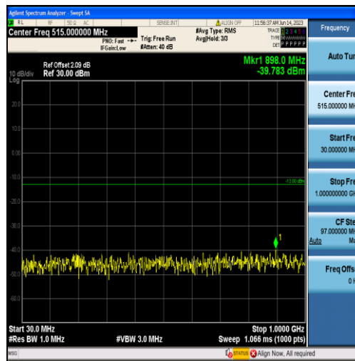
Band2-5MHz-16QAM-19175-25RB#0-Range1:30~1000MHz
