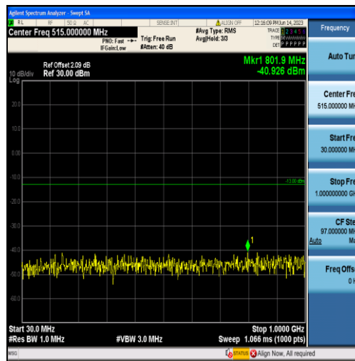
Band2-15MHz-QPSK-18900-75RB#0-Range1:30~1000MHz
