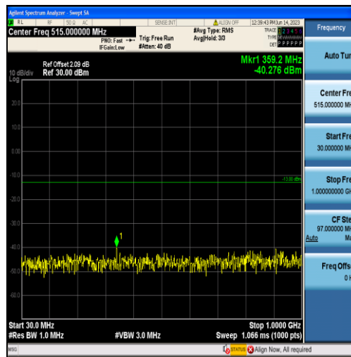
Band4-1.4MHz-16QAM-20393-6RB#0-Range1:30~1000MHz
