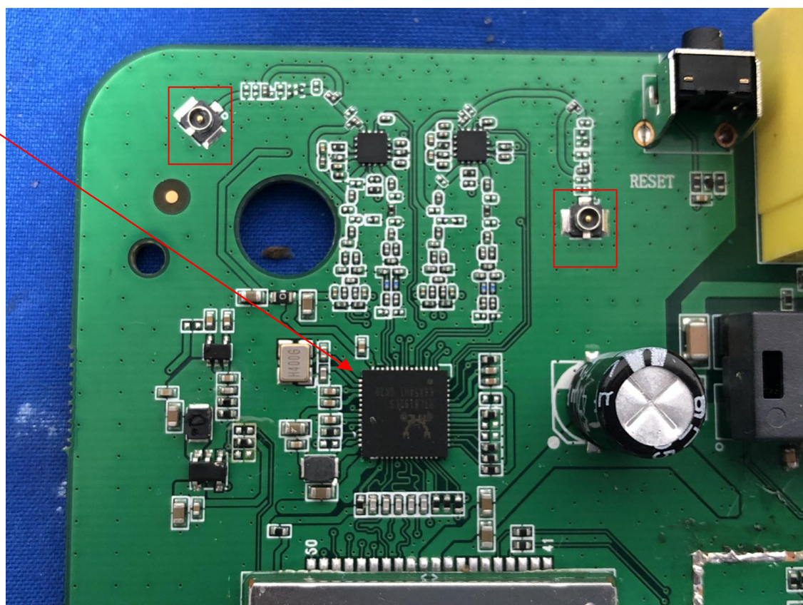
2.4G Wifi antenna
