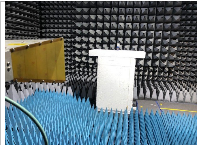
Fig 3 Test setup 1GHz 18GHz Rad Emissions
