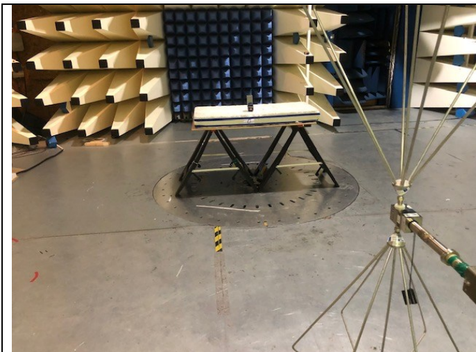
Fig 1b Test setup 30MHz -300MHz Rad Emissions
