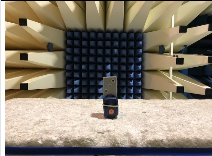
Fig 5a EUT close up Rad Emissions
