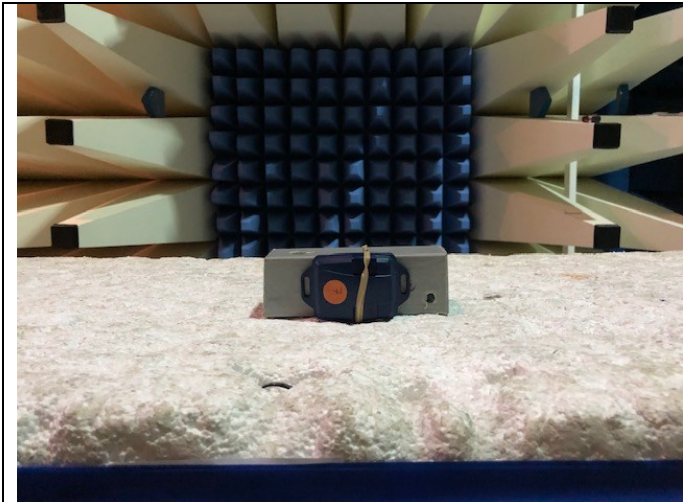
Fig 5b EUT close up Rad Emissions
