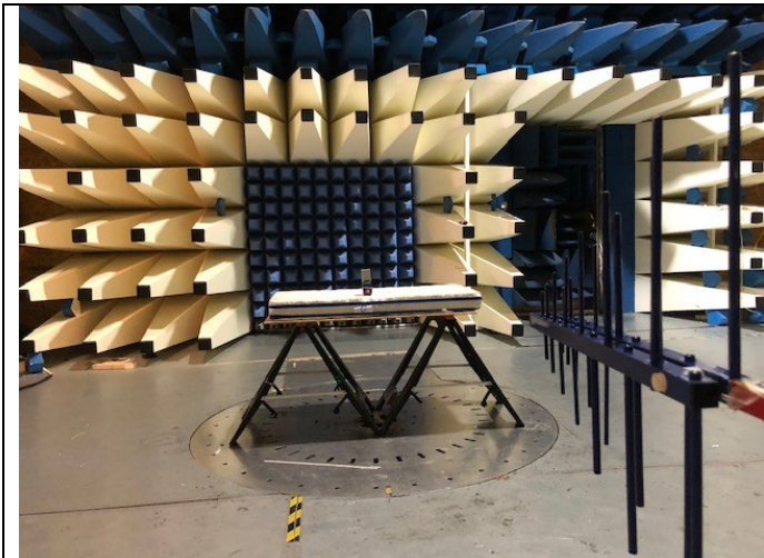
Fig 2b Test setup 300MHz -1GHz Rad Emissions
