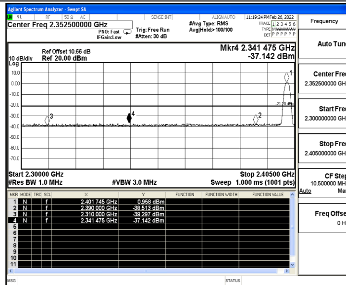
BLE_1M_Ant_High_2480_AV
