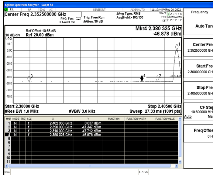
BLE_1M_Ant_Low_2402_Peak
