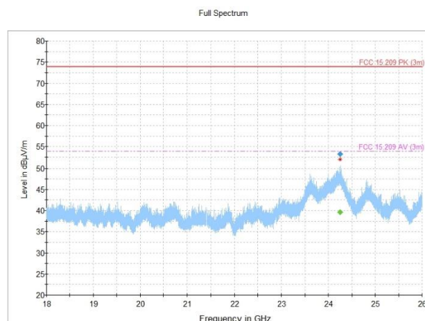
Figure 8.2-21: Radiated spurious emissions, 802.11g, low channel
