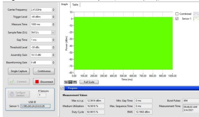
Figure 8.1-3: Maximum conducted power, 802.11n (SISO), low channel
