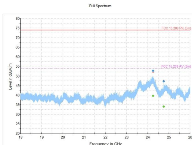
Figure 8.2-26: Radiated spurious emissions, 802.11n, MIMO antenna configuration, high channel
