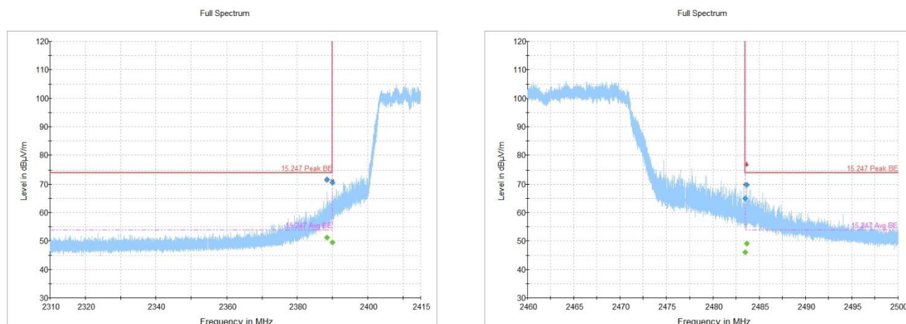
Figure 8.2-4: Radiated emissions, restricted band edge, 802.11n, MIMO antenna configuration
