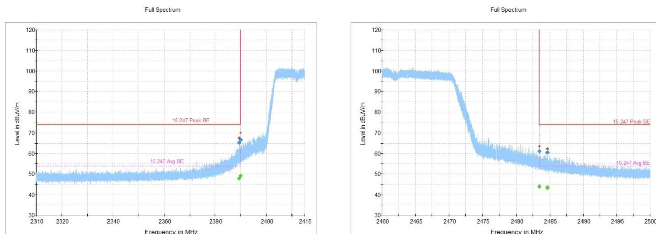
Figure 8.2-3: Radiated emissions, restricted band edge, 802.11n, SISO antenna configuration
