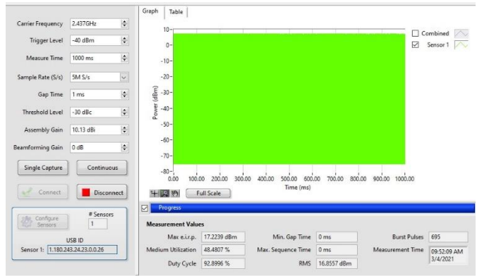
Figure 8.1-4: Maximum conducted power, 802.11n (SISO), mid channel
