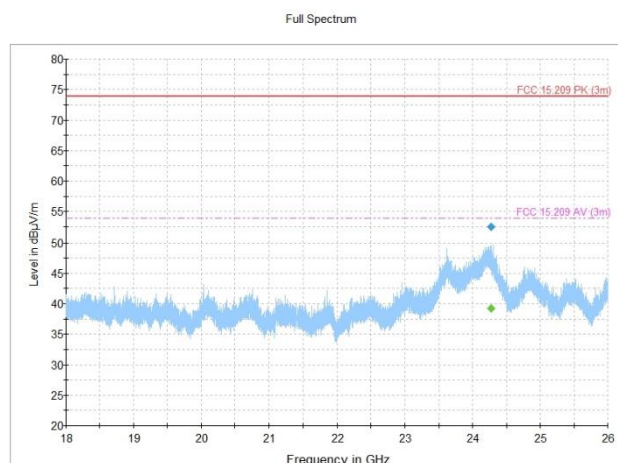
Figure 8.2-18: Radiated spurious emissions, 802.11b, low channel
