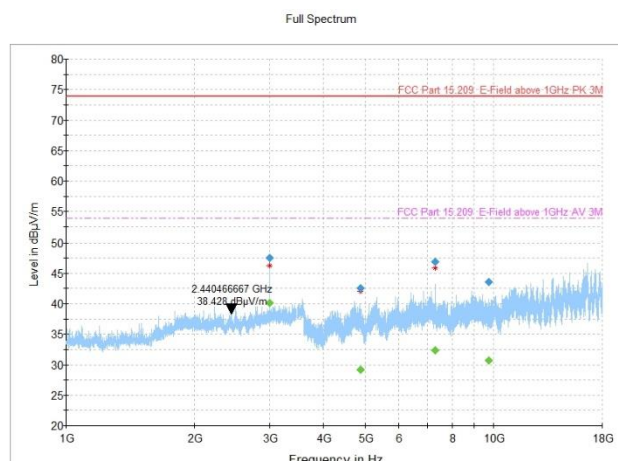
Figure 8.2-16: Radiated spurious emissions, 802.11n, MIMO antenna configuration, mid channel
