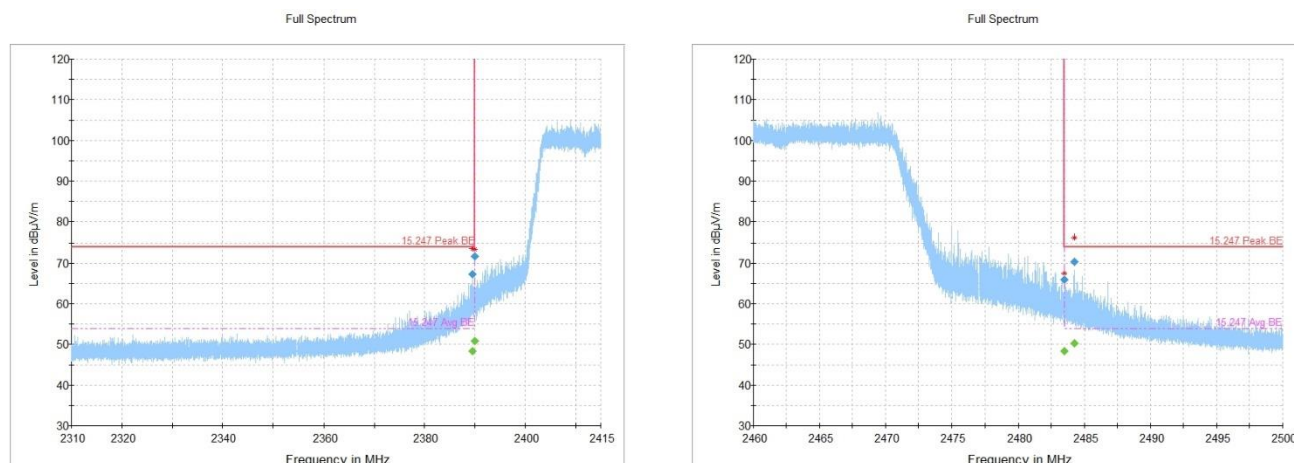
Figure 8.2-6: Radiated emissions, restricted band edge, 802.11ac, MIMO antenna configuration
