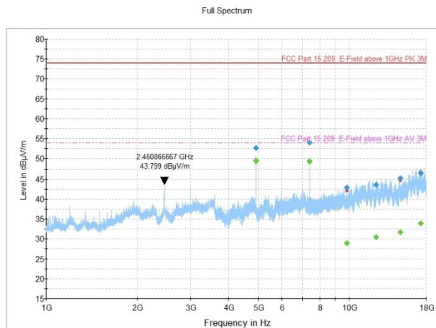
Figure 8.2-10: Radiated spurious emissions, 802.11b, high channel
