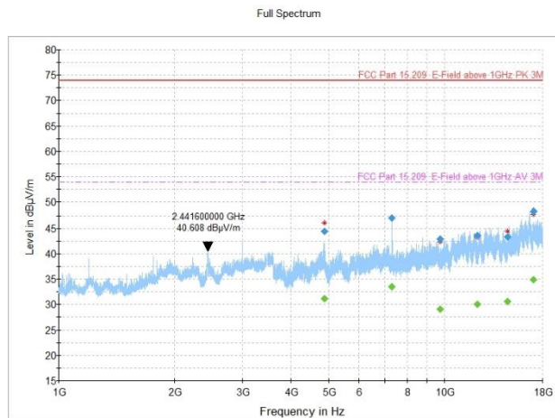
Figure 8.2-14: Radiated spurious emissions, 802.11n, SISO antenna configuration, mid channel
