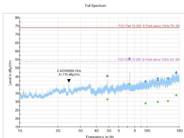
Figure 8.2-12: Radiated spurious emissions, 802.11g, mid channel
