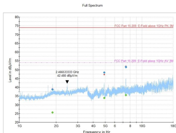
Figure 8.2-13: Radiated spurious emissions, 802.11g, high channel
