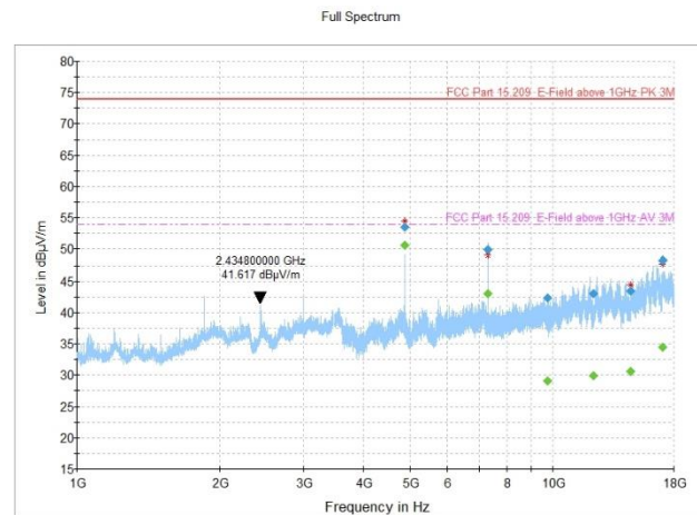
Figure 8.2-9: Radiated spurious emissions, 802.11b, mid channel
