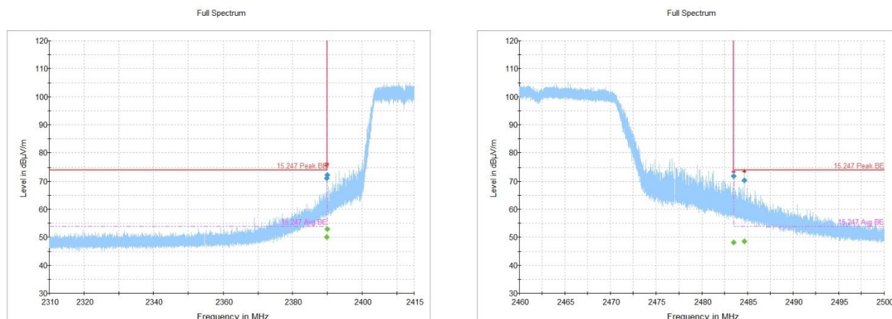
Figure 8.2-5: Radiated emissions, restricted band edge, 802.11ac, SISO antenna configuration
