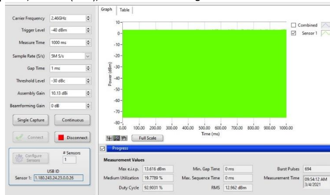
Figure 8.1-5: Maximum conducted power, 802.11n (SISO), high channel
