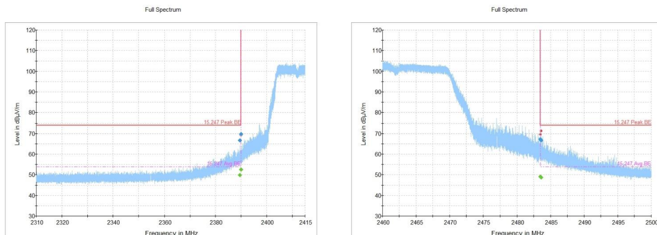
Figure 8.2-2: Radiated emissions, restricted band edge, 802.11g
