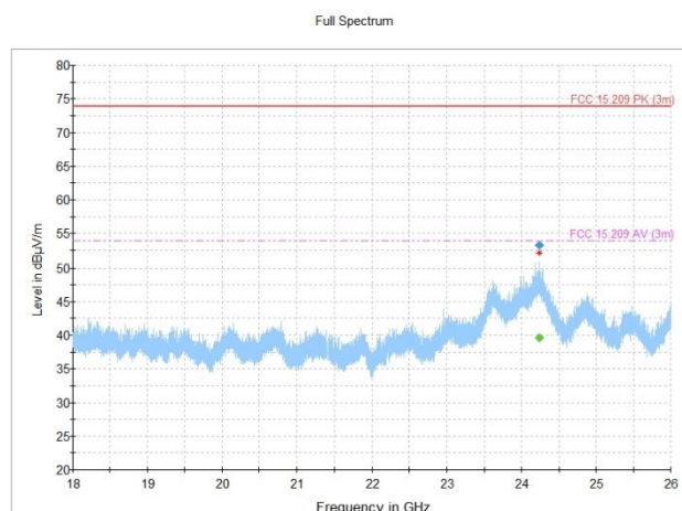
Figure 8.2-24: Radiated spurious emissions, 802.11n, MIMO antenna configuration, low channel
