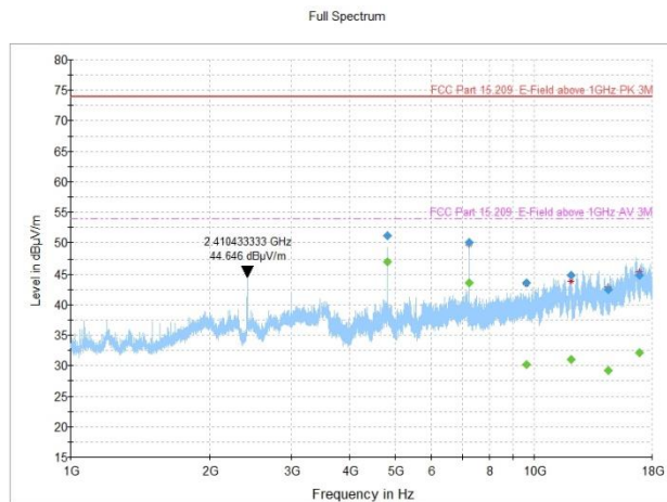
Figure 8.2-8: Radiated spurious emissions, 802.11b, low channel
