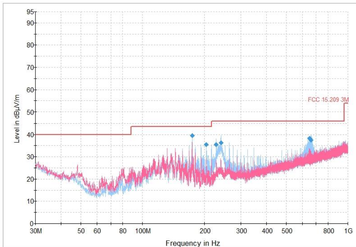
Figure 8.2-7: Radiated emissions, 802.11n, MIMO antenna configuration, mid channel, 30 – 1000 MHz spectral plot
