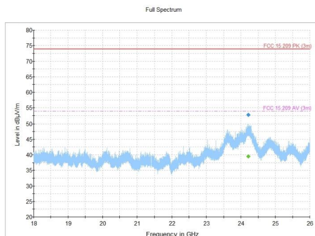
Figure 8.2-20: Radiated spurious emissions, 802.11b, high channel
