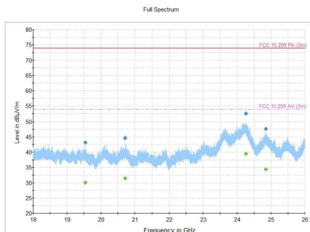
Figure 8.2-22: Radiated spurious emissions, 802.11g, mid channel
