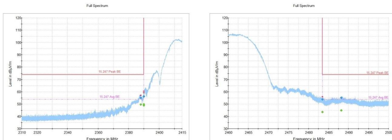
Figure 8.2-1: Radiated emissions, restricted band edge, 802.11b
