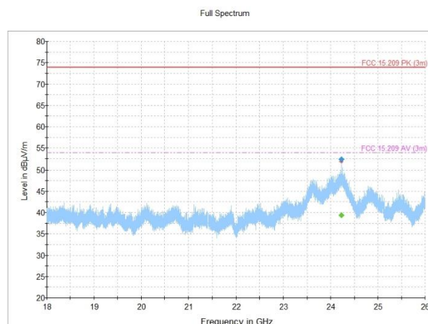
Figure 8.2-23: Radiated spurious emissions, 802.11g, high channel
