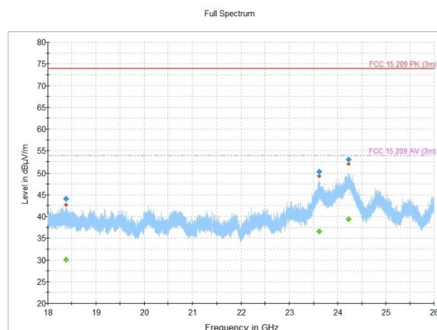
Figure 8.2-19: Radiated spurious emissions, 802.11b, mid channel
