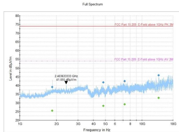
Figure 8.2-15: Radiated spurious emissions, 802.11n, MIMO antenna configuration, low channel
