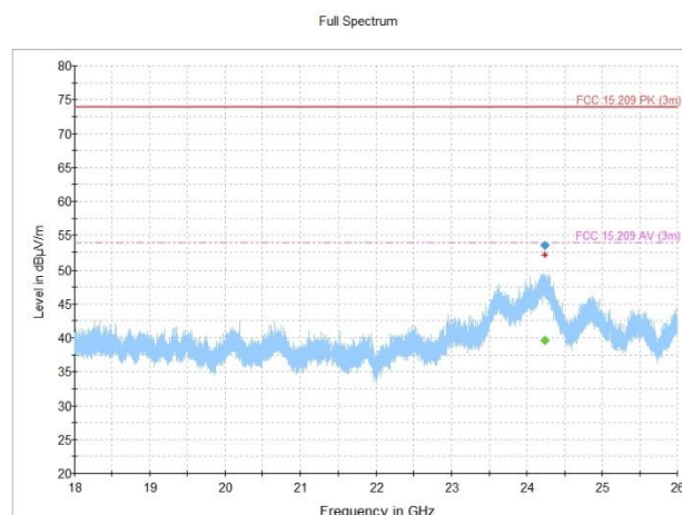
Figure 8.2-25: Radiated spurious emissions, 802.11n, MIMO antenna configuration, mid channel
