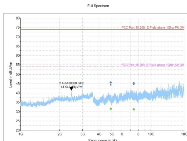
Figure 8.2-17: Radiated spurious emissions, 802.11n, MIMO antenna configuration, high channel
