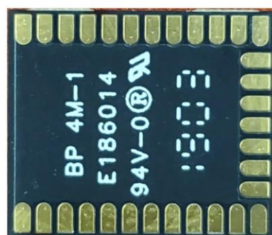
Figure2: External, Bottom View
