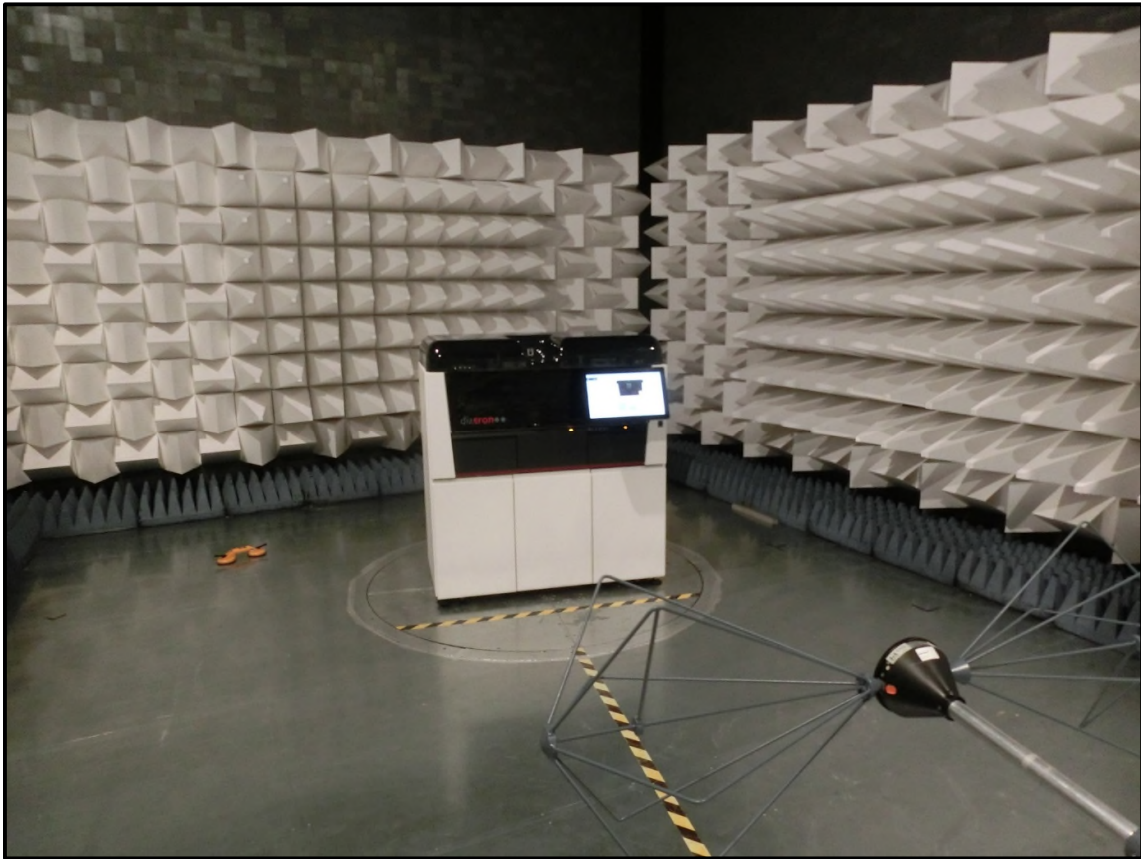
Radiated Spurious Emission from 30 MHz to 200 MHz
