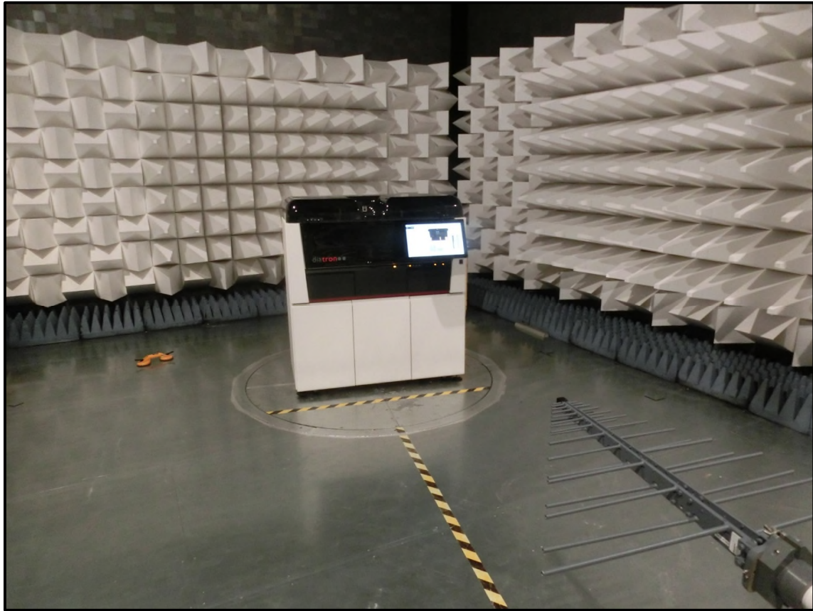
Radiated Spurious Emission from 200 MHz to 1000 MHz
