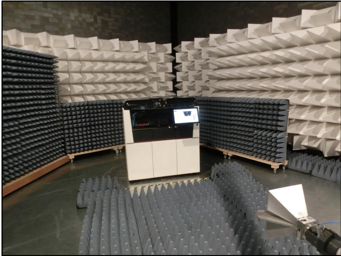
Radiated Spurious Emission above 1GHz
