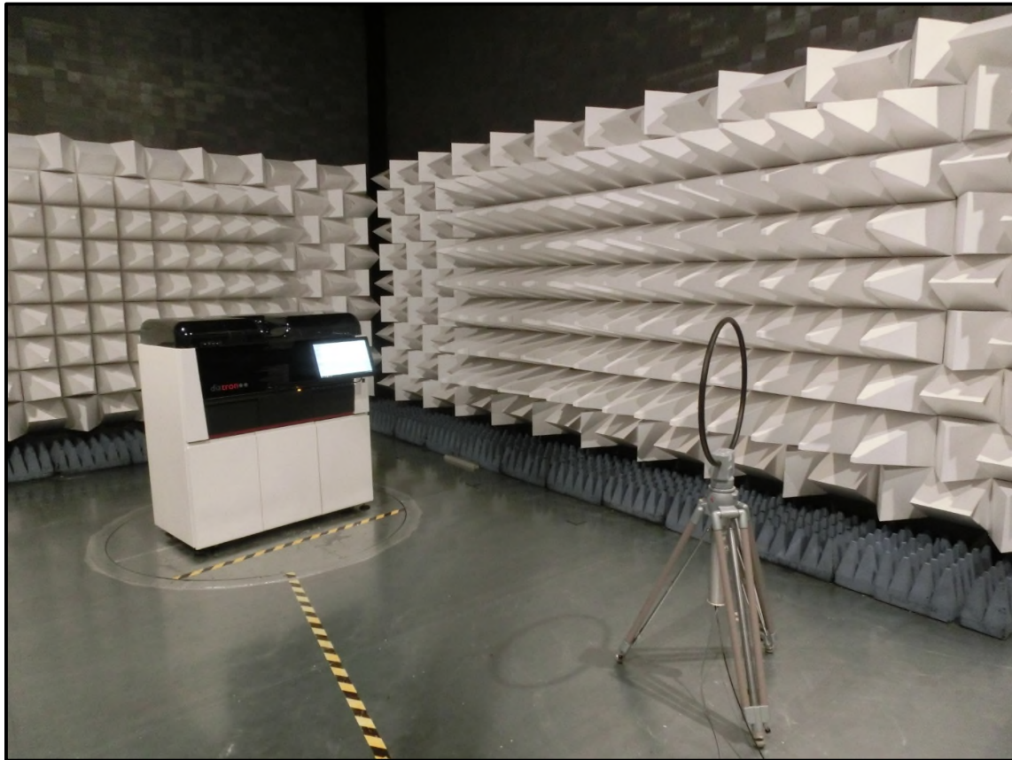
Radiated Spurious Emissions from 9 kHz to 30MHz
