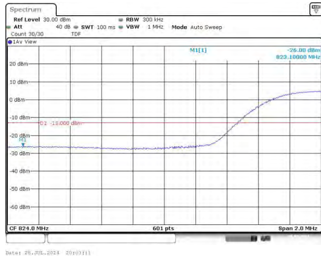
Band26-15MHz-16QAM-26965-75RB#0
