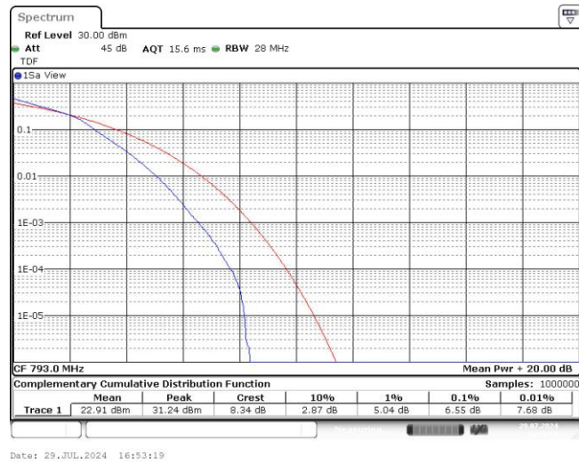
Band14-5MHz-16QAM-23355-1RB#0
