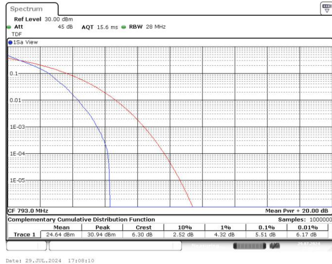
Band14-10MHz-QPSK-23330-50RB#0
