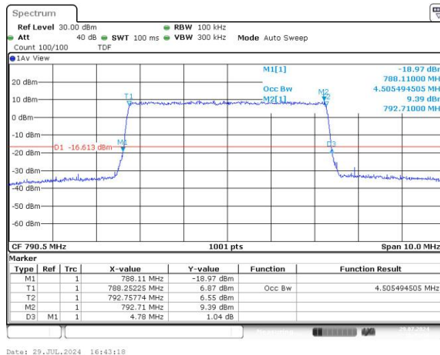
Band14-5MHz-16QAM-23330-25RB#0
