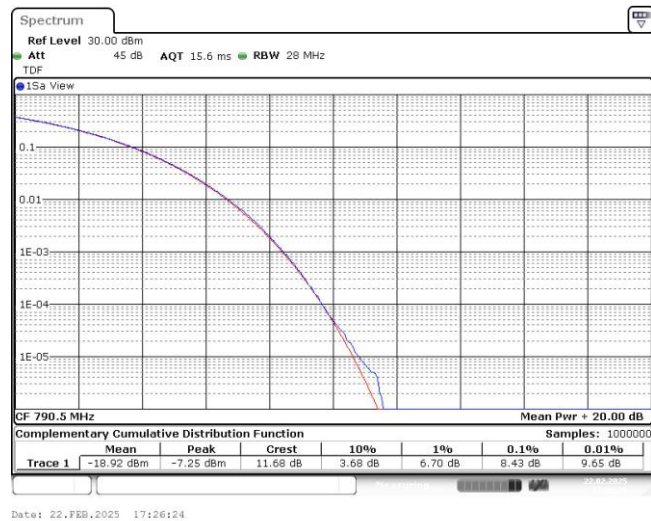
Band14-5MHz-QPSK-23330-1RB#0
