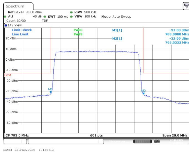
Band14-10MHz-16QAM-23330-1RB#0
