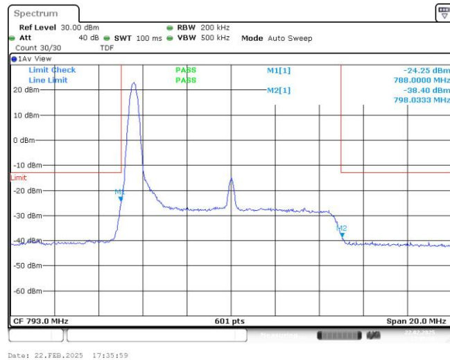
Band14-10MHz-16QAM-23330-50RB#0
