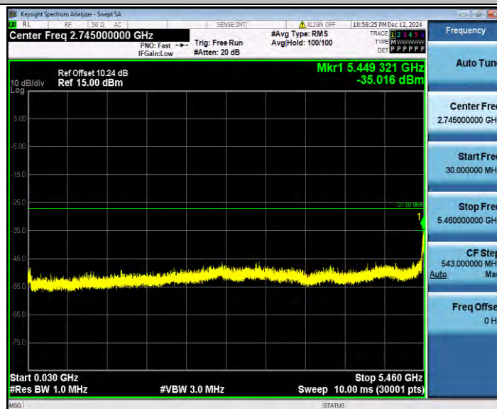
11AX40SISO_Ant1_5670_30~5460
