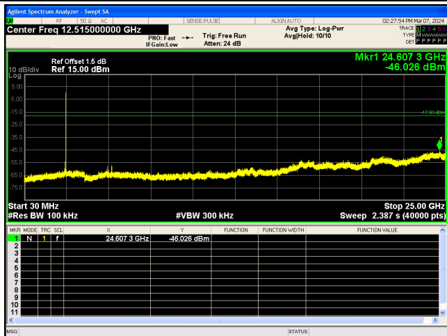
8-DPSK_2402_0~Reference
