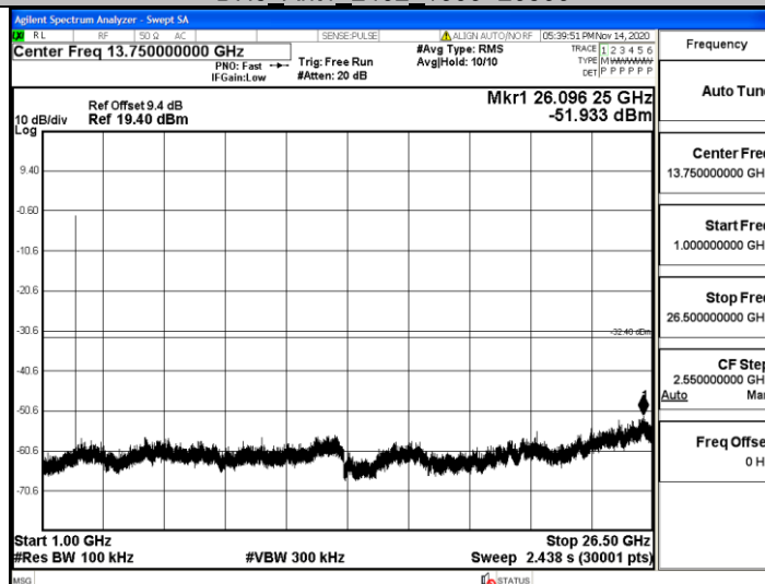
DH5_Ant1_2441_0~Reference
