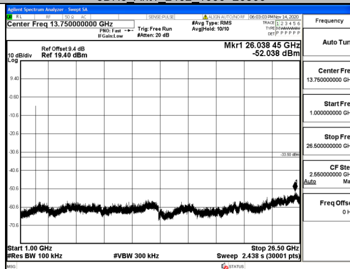
3DH5_Ant1_2441_0~Reference
