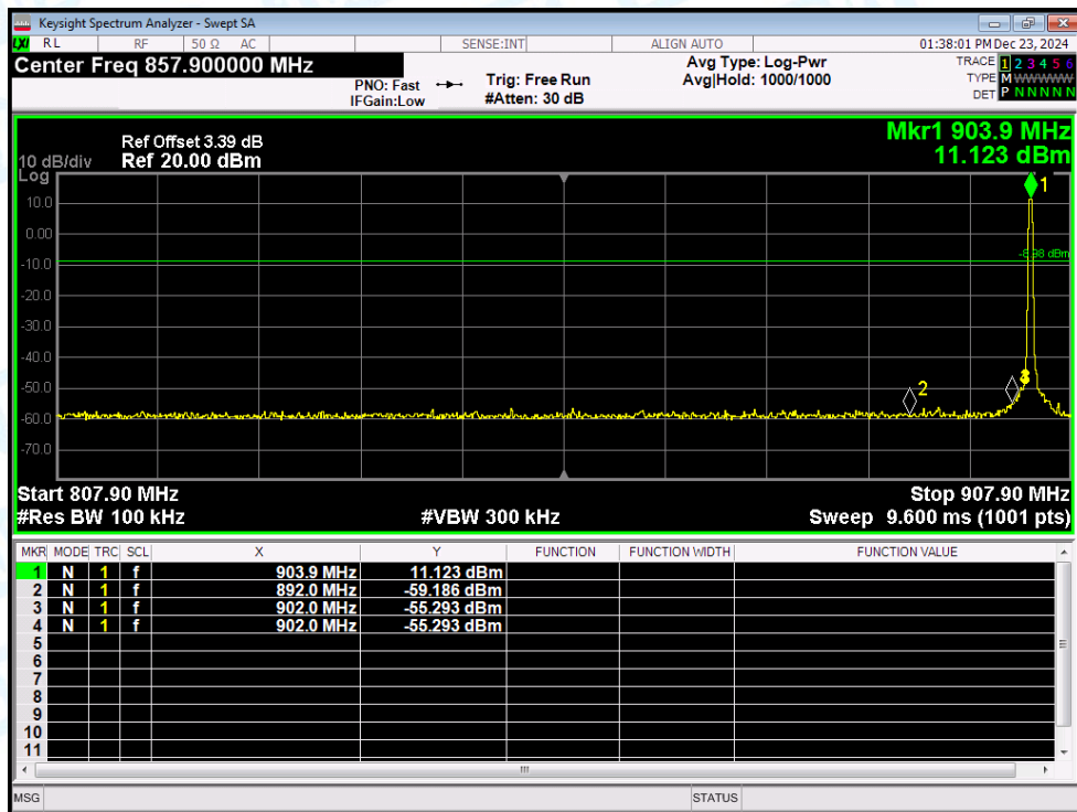
Band Edge NVNT LoRa 903.9MHz Ant1 Emission
