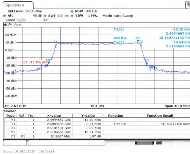
Band7-20MHz-16QAM-21100-100RB#0-18.17
