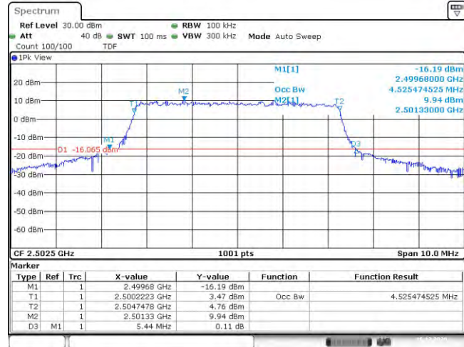
Band7-5MHz-QPSK-20775-25RB#0-4.525
