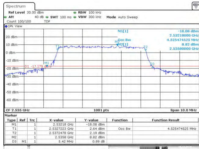
Band7-5MHz-QPSK-21100-25RB#0-4.525
