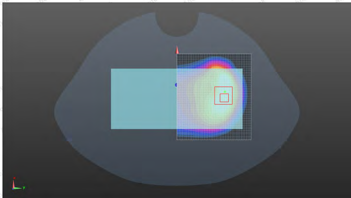
Figure 14: LTE Band 5_QPSK _Rear side
