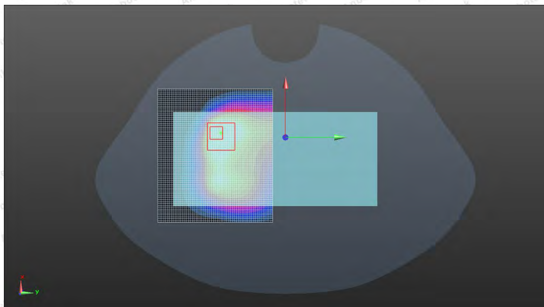
Figure 16: WLAN 2.4G_Rear side_0mm
