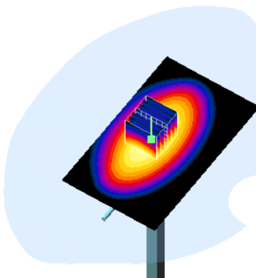
System Performance Check 835MHz Head 250mW
