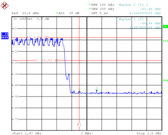
Hopping Band edge-right side
