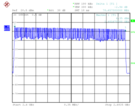
Modulation: GFSK
