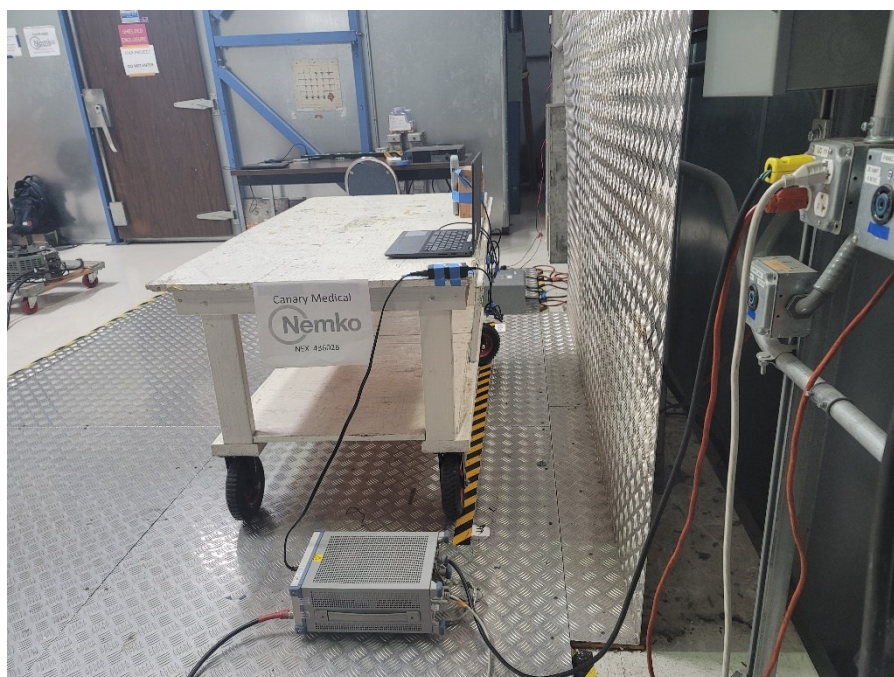
Figure 7 – Test setup, side view.
