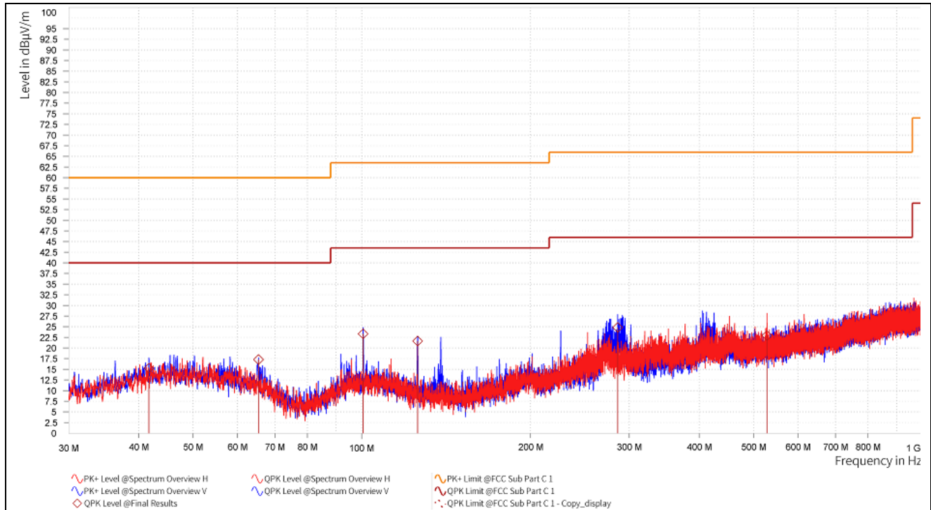
30 MHz – 1 GHz
