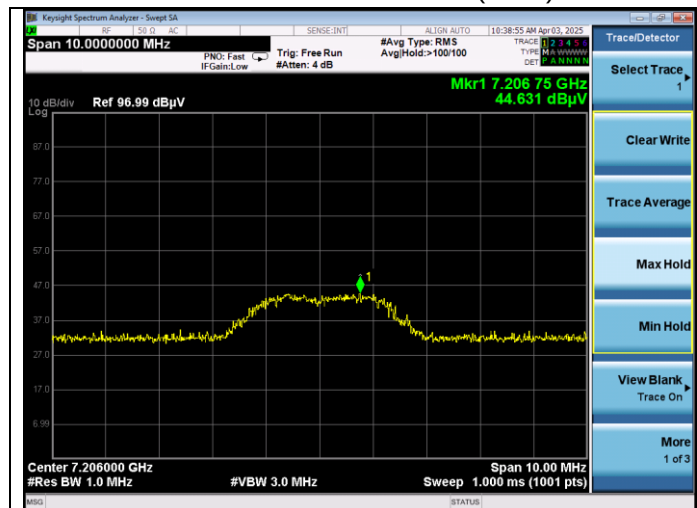
Low channel 3 rd harmonic (Peak)
