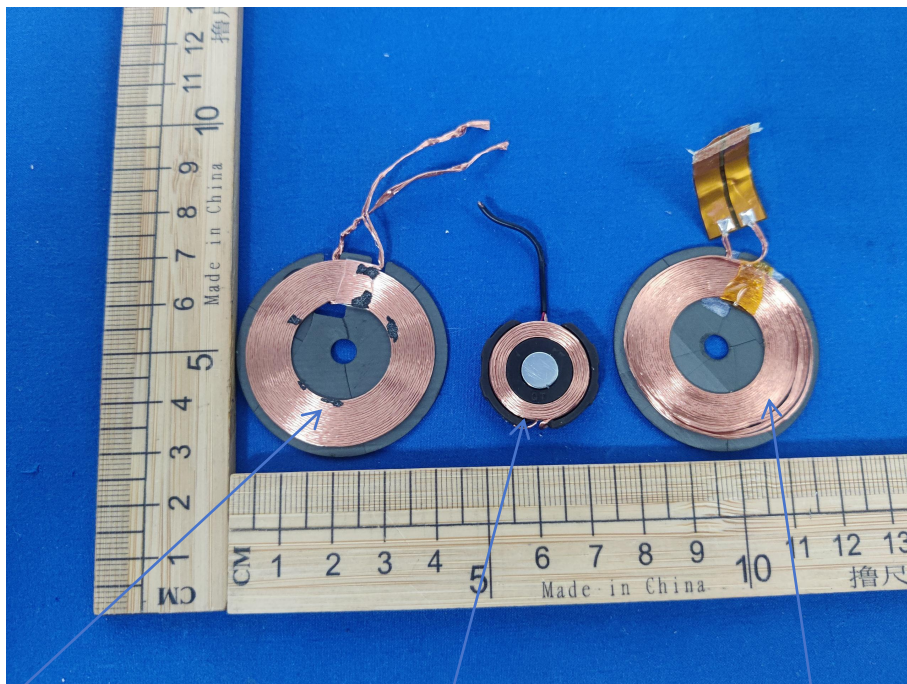
ANT 43.5-7mm Coil specification
