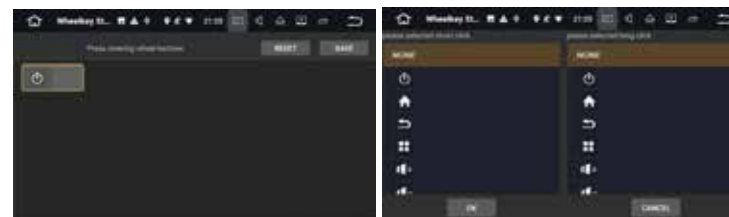
UI(1)
