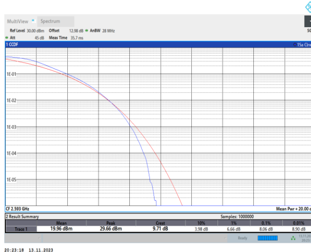
Band41-20MHz-QPSK-40620-100RB#0
