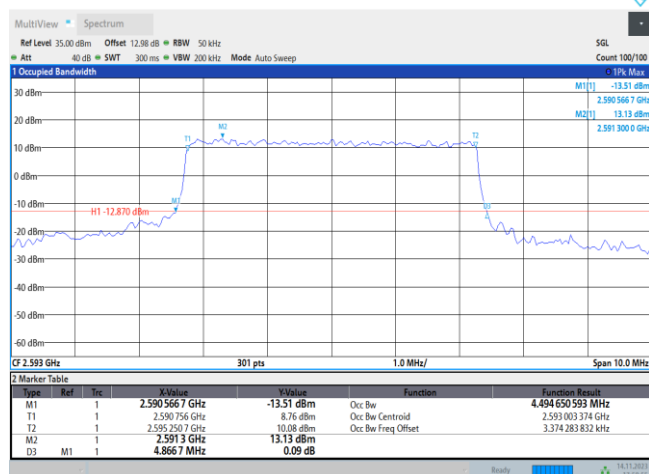
Band41-5MHz-QPSK-40620-25RB#0
