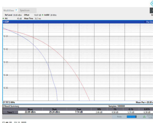
Band12-10MHz-QPSK-23095-50RB#0
