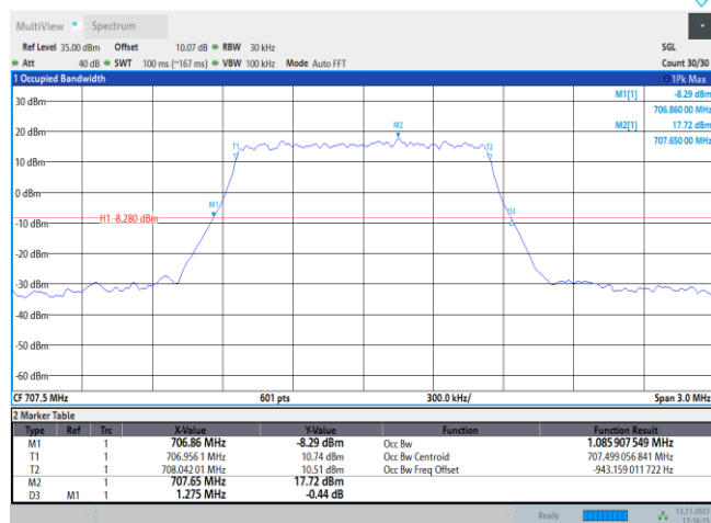
Band12-1.4MHz-QPSK-23095-6RB#0
