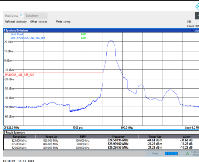
Band5-1.4MHz-QPSK-20427-6RB#0
