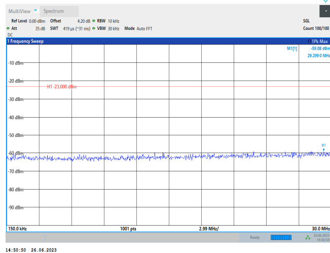
Band17-10MHz-QPSK-23780-1RB#0-Range2:0.15~30MHz
