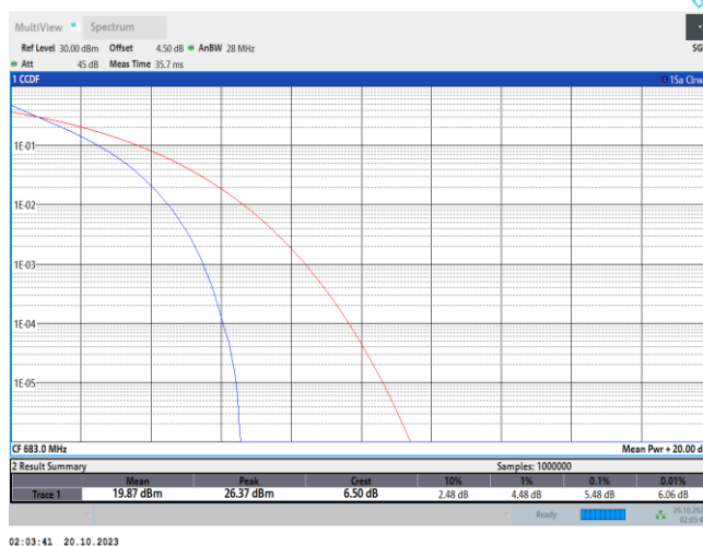
Band71-20MHz-QPSK-133322-100RB#0
