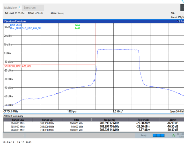
Band17-5MHz-QPSK-23755-25RB#0
