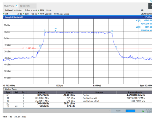
Band17-5MHz-16QAM-23790-25RB#0
