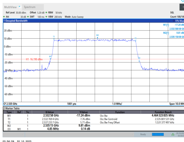
Band7-5MHz-16QAM-21100-25RB#0
