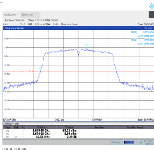
11ac40SISO-Ant9-5670
