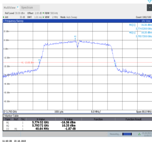
11ac40SISO-Ant9-5795
