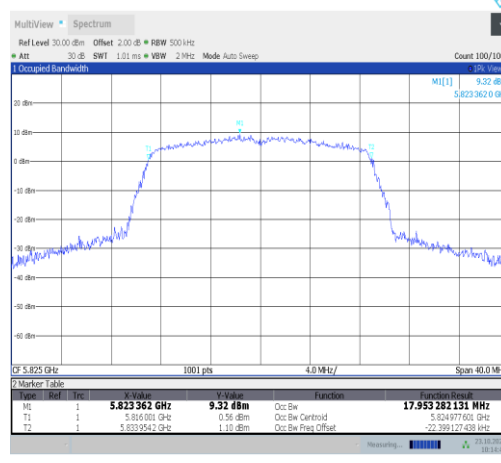
11ac20SISO-Ant9-5825
