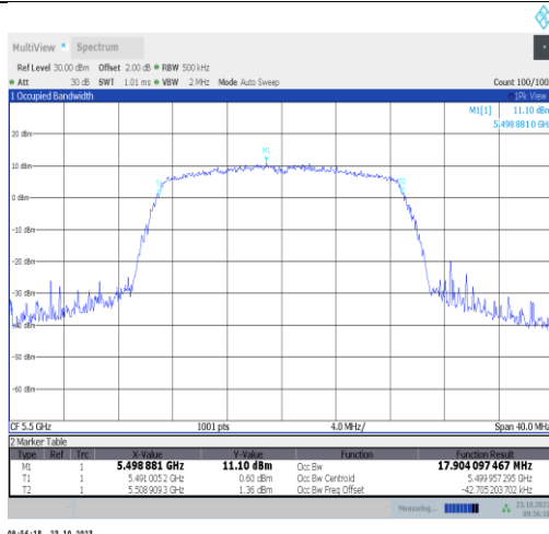
11ac20SISO-Ant9-5500
