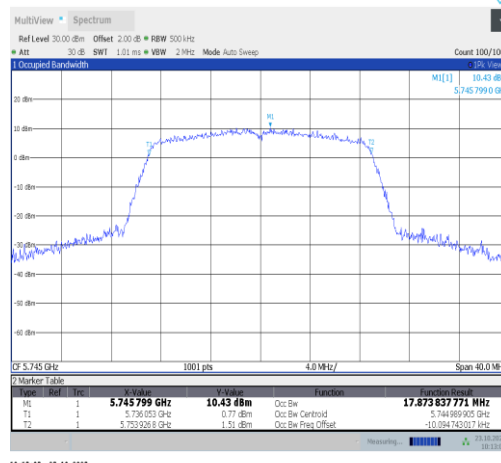
11ac20SISO-Ant9-5745
