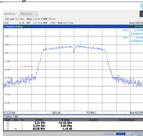
11ac40SISO-Ant9-5230
