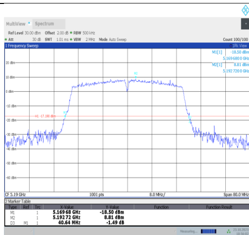
11ac40SISO-Ant9-5190
