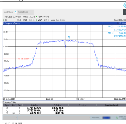
11ac40SISO-Ant9-5755
