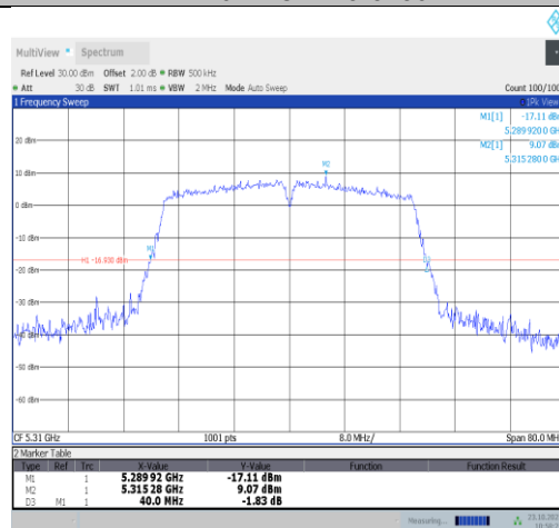
11ac40SISO-Ant9-5310
