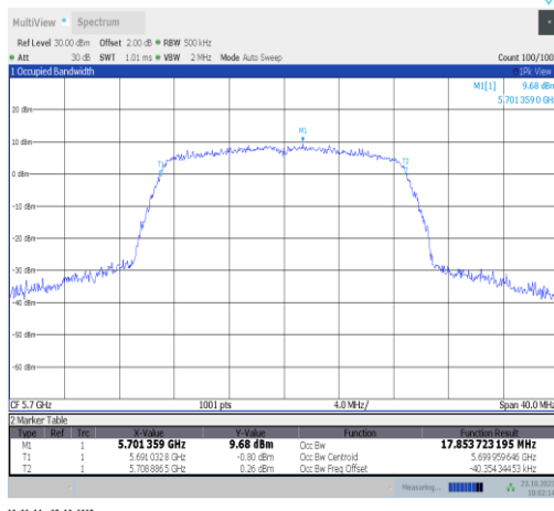
11ac20SISO-Ant9-5700
