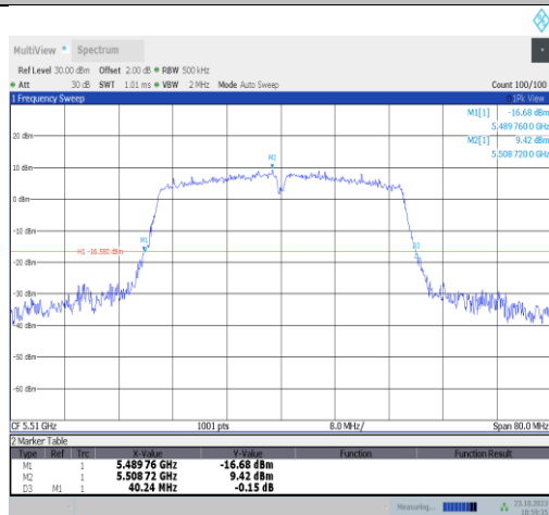
11ac40SISO-Ant9-5510
