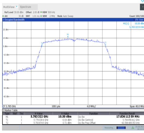
11ac20SISO-Ant9-5785
