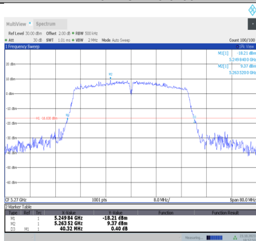
11ac40SISO-Ant9-5270
