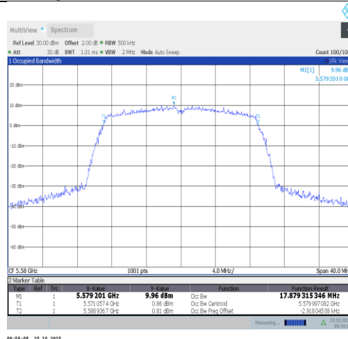
11ac20SISO-Ant9-5580
