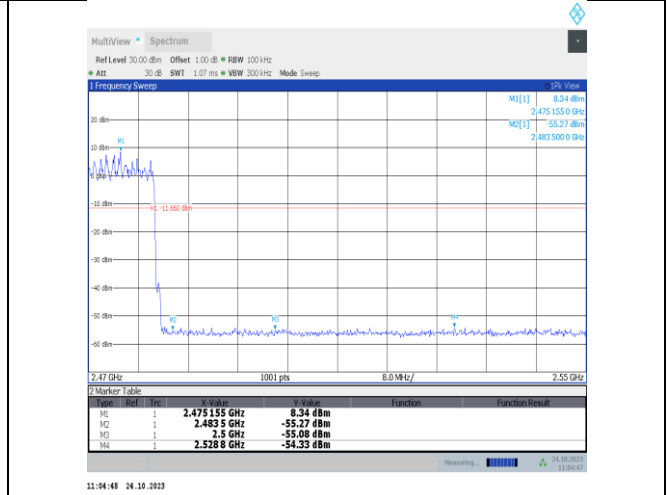
2DH5-Ant9-Hop_2480-PASS
