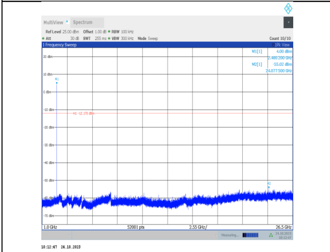
3DH5-Ant9-2480-1000~26500-PASS
