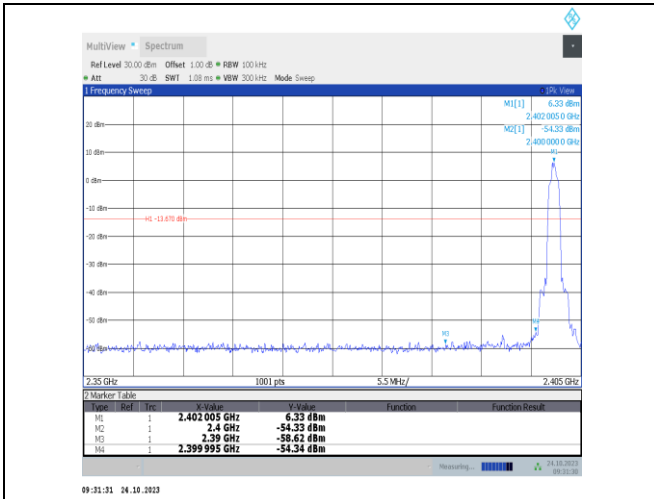
2DH5-Ant9-2402-PASS
