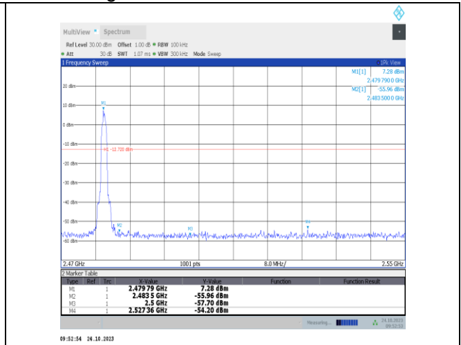
2DH5-Ant9-2480-PASS
