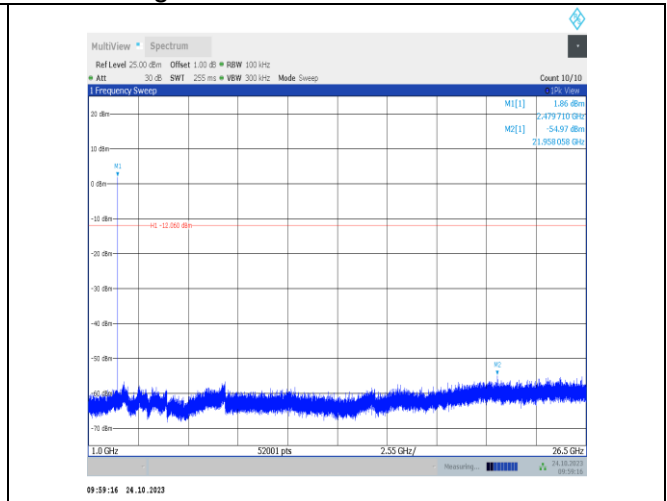
2DH5-Ant9-2480-1000~26500-PASS
