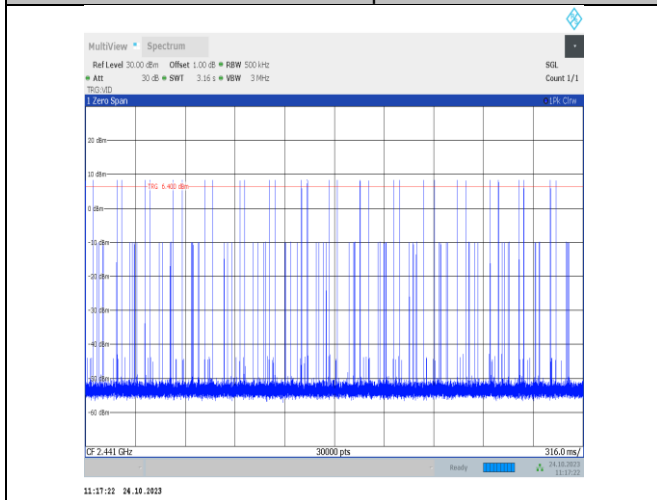
3DH1-Ant9-Hop-PASS
