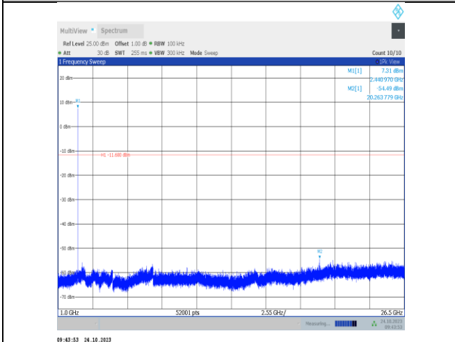
2DH5-Ant9-2441-1000~26500-PASS
