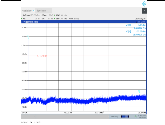
DH5-Ant9-2480-1000~26500-PASS
