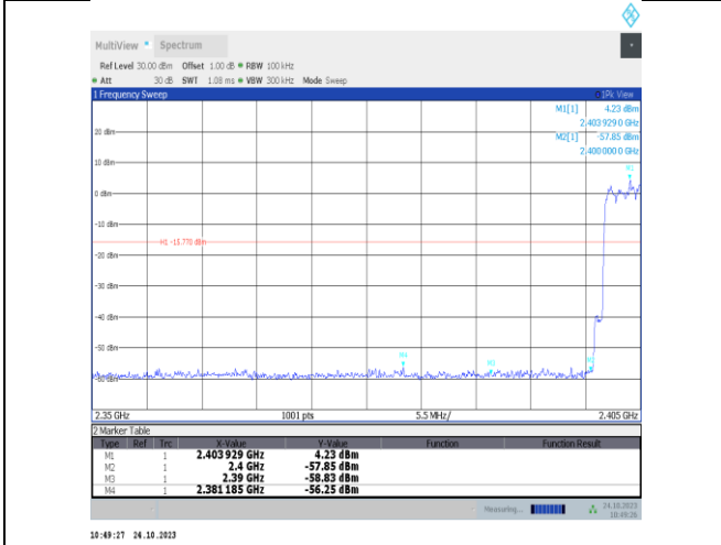
2DH5-Ant9-Hop_2402-PASS
