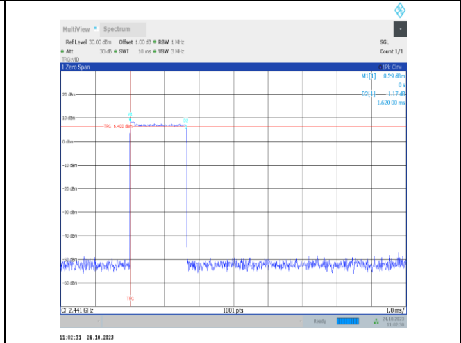
2DH3-Ant9-Hop-PASS
