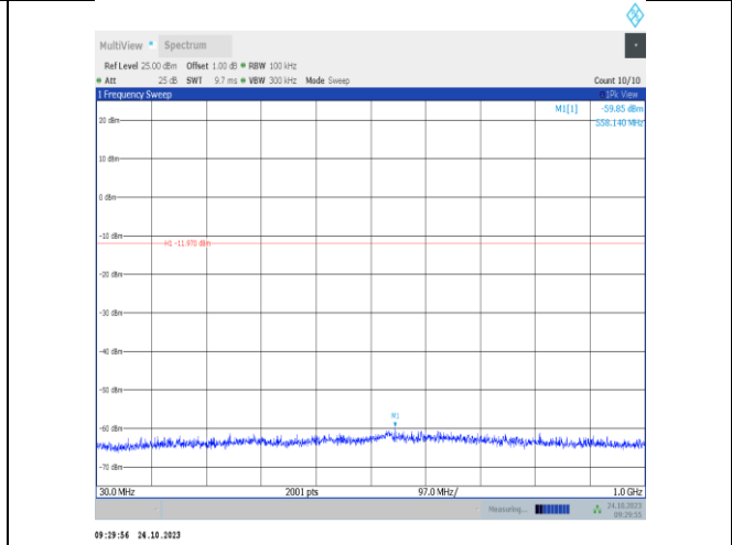
DH5-Ant9-2480-30~1000-PASS
