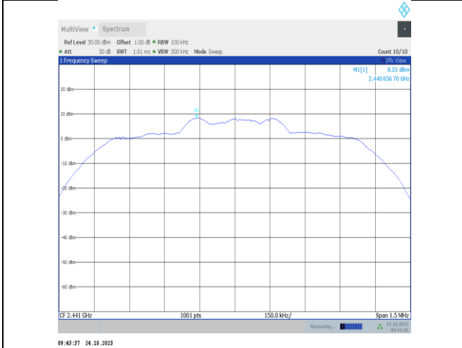
2DH5-Ant9-2441-0~Reference-PASS
