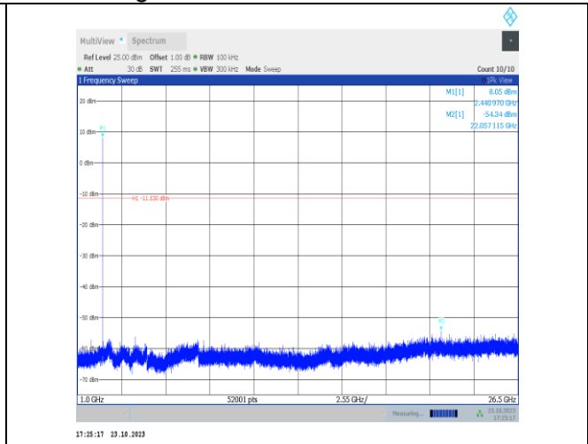
DH5-Ant9-2441-1000~26500-PASS
