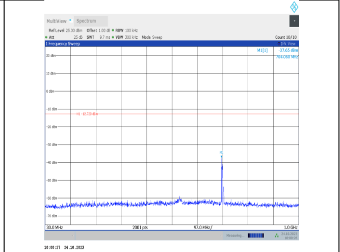
3DH5-Ant9-2402-30~1000-PASS
