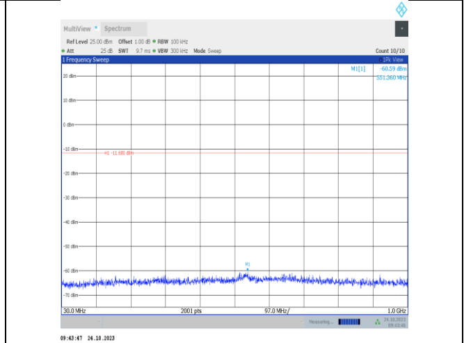
2DH5-Ant9-2441-30~1000-PASS
