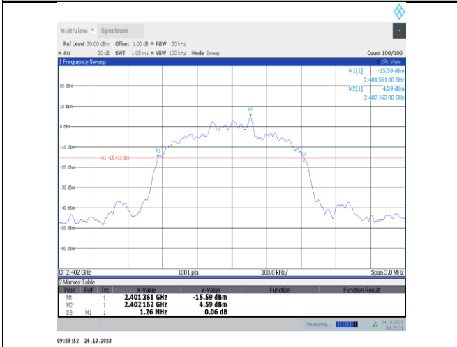
3DH5-Ant9-2402
