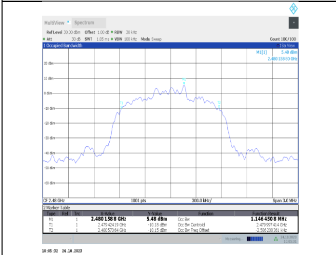
3DH5-Ant9-2480
