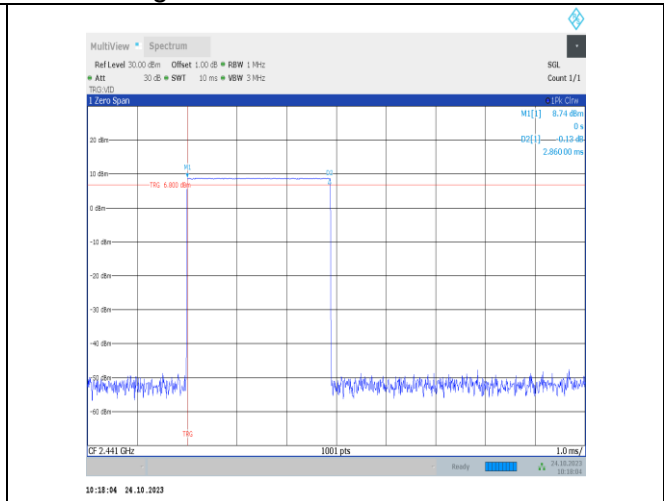
DH5-Ant9-Hop-PASS
