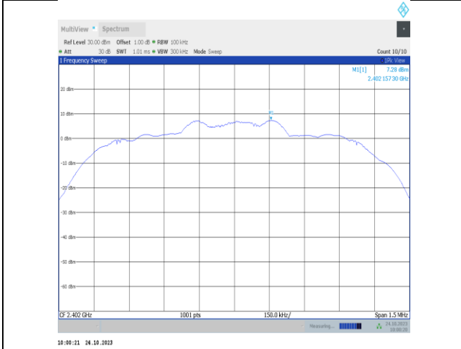
3DH5-Ant9-2402-0~Reference-PASS
