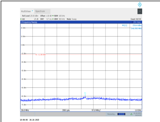
3DH5-Ant9-2441-30~1000-PASS
