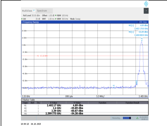
3DH5-Ant9-2402-PASS
