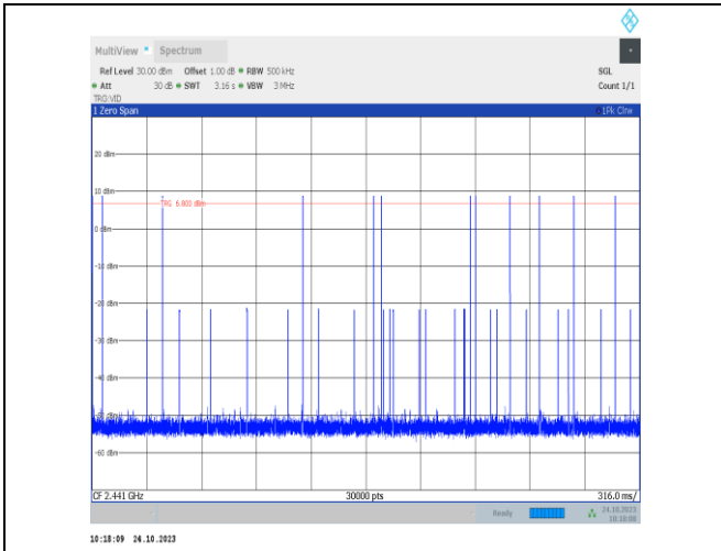
DH5-Ant9-Hop-PASS
