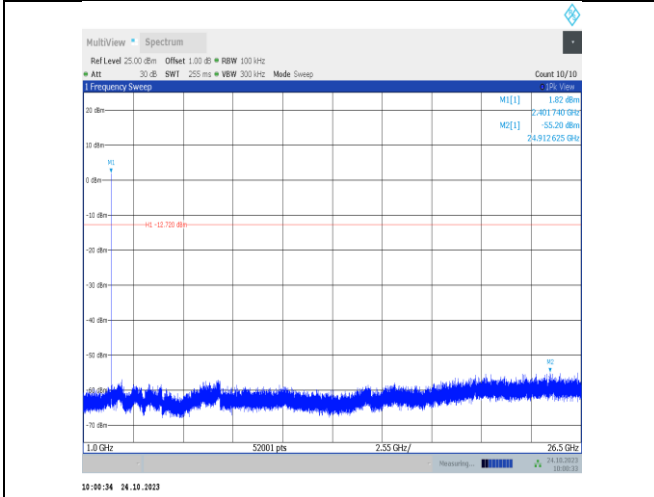
3DH5-Ant9-2402-1000~26500-PASS
