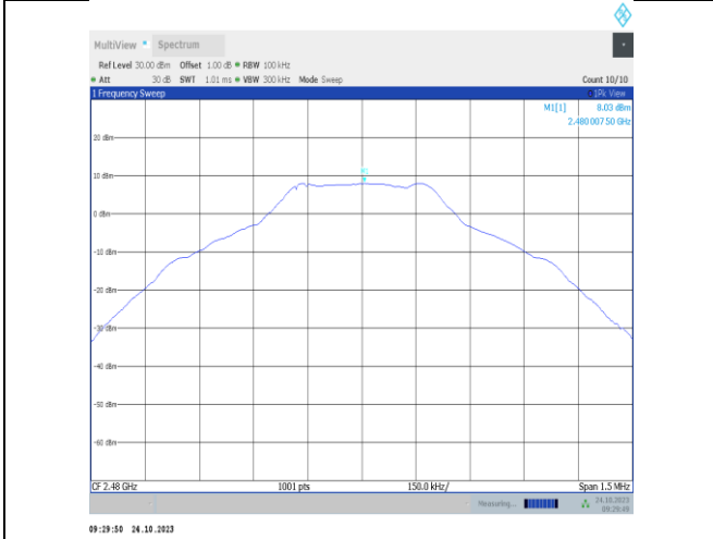
DH5-Ant9-2480-0~Reference-PASS
