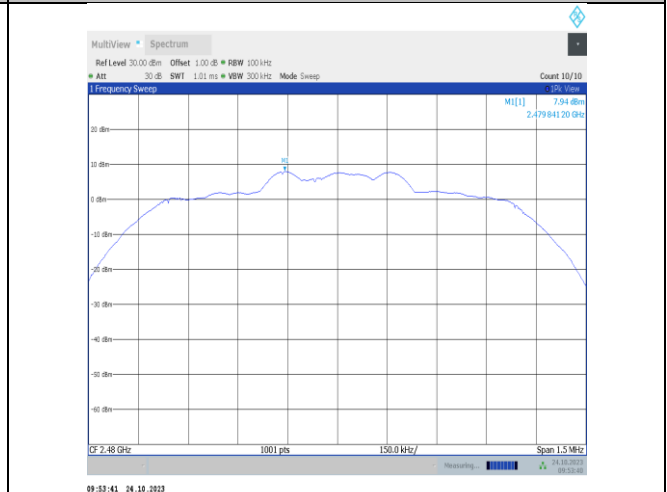
2DH5-Ant9-2480-0~Reference-PASS
