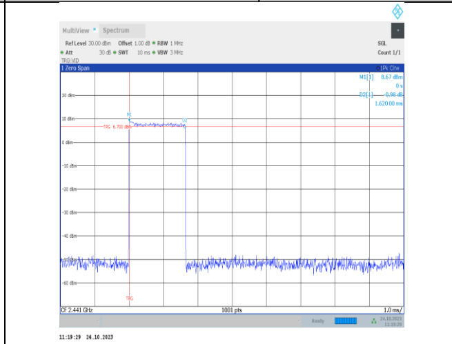
3DH3-Ant9-Hop-PASS
