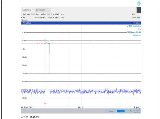
2DH1-Ant9-Hop-PASS
