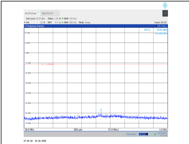
DH5-Ant9-2441-30~1000-PASS
