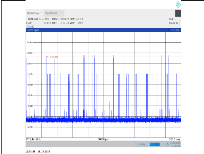
2DH3-Ant9-Hop-PASS
