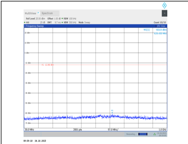
2DH5-Ant9-2480-30~1000-PASS
