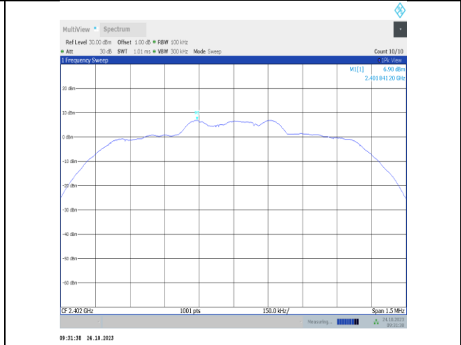
2DH5-Ant9-2402-0~Reference-PASS
