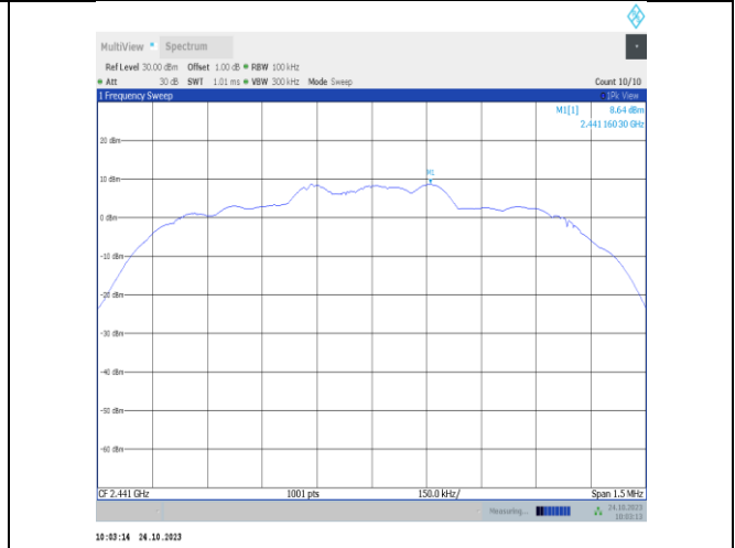
3DH5-Ant9-2441-0~Reference-PASS
