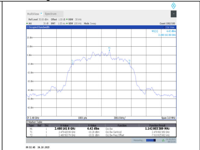
2DH5-Ant9-2480
