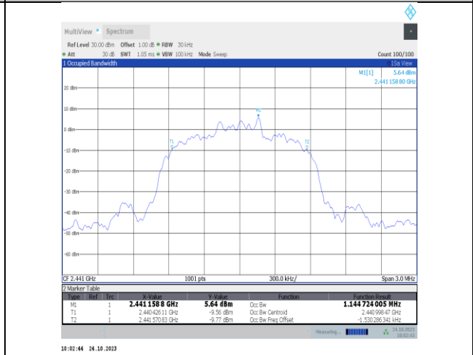
3DH5-Ant9-2441
