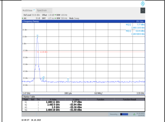
3DH5-Ant9-2480-PASS
