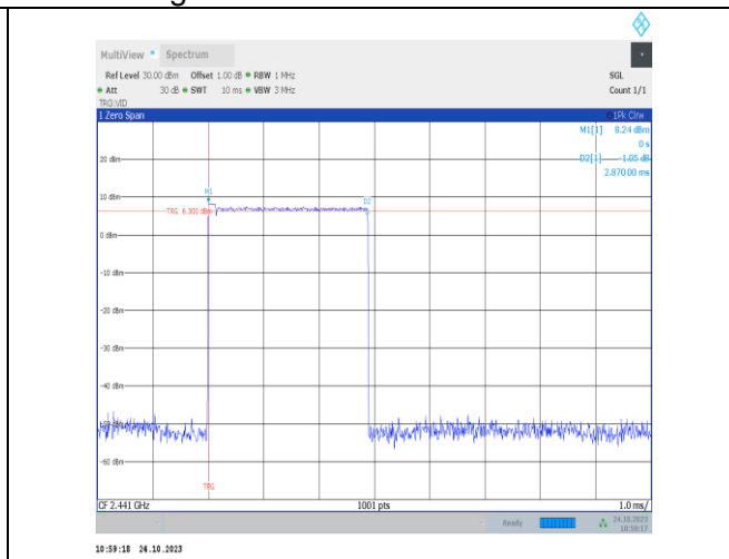
2DH5-Ant9-Hop-PASS
