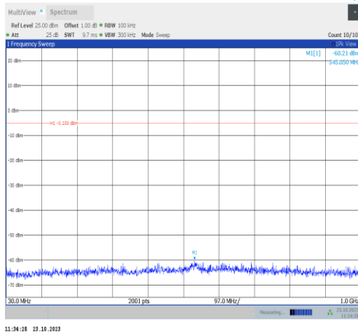
11b-Ant9-2437-30~1000-PASS
