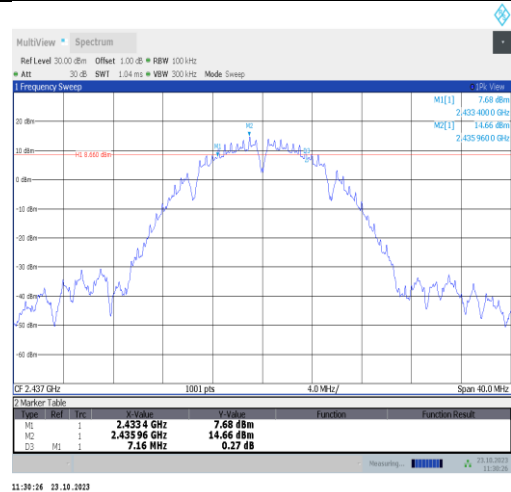
11b-Ant9-2437-PASS
