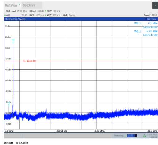
11g-Ant9-2462-1000~26500-PASS
