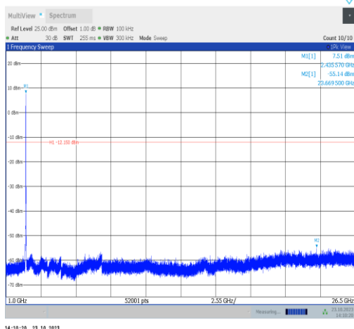
11g-Ant9-2437-1000~26500-PASS
