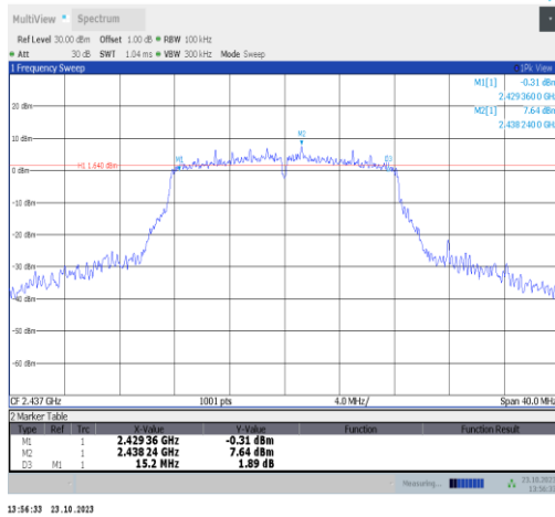
11g-Ant9-2437-PASS
