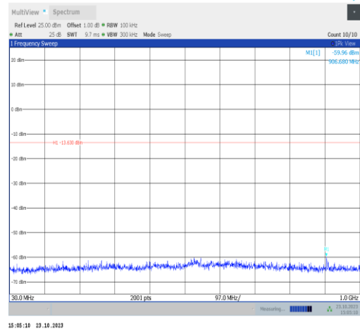
11n20SISO-Ant9-2412-30~1000-PASS
