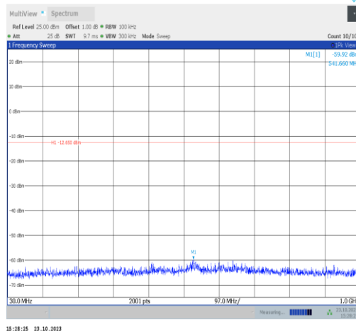
11n20SISO-Ant9-2462-30~1000-PASS
