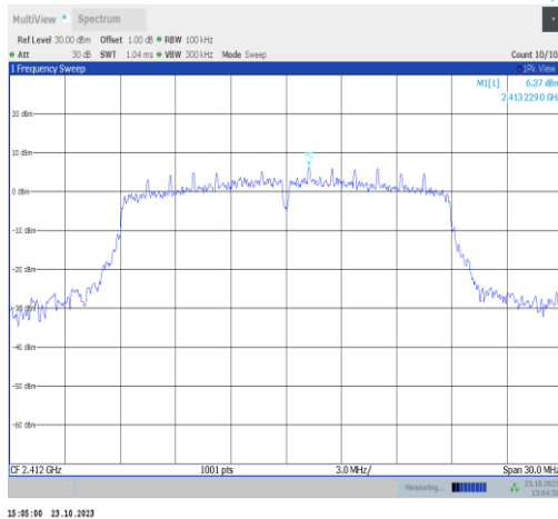
11n20SISO-Ant9-2412-0~Reference-PASS
