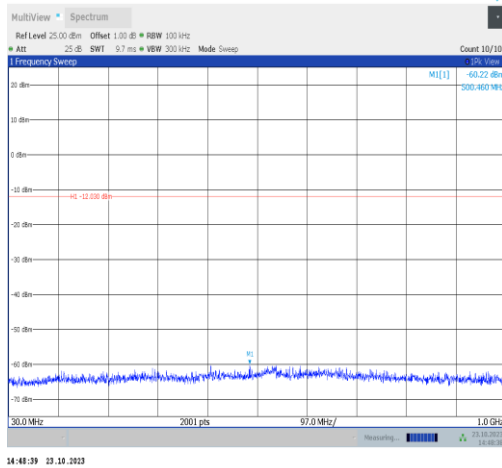
11g-Ant9-2462-30~1000-PASS
