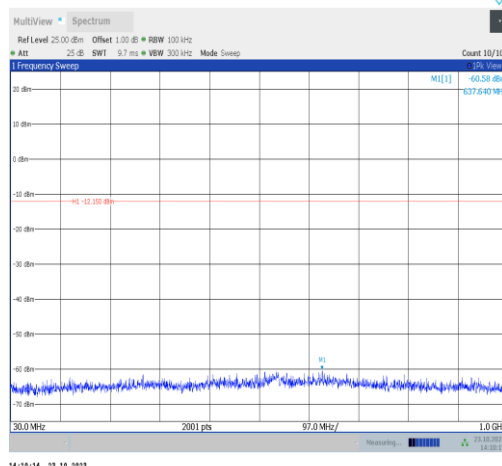
11g-Ant9-2437-30~1000-PASS
