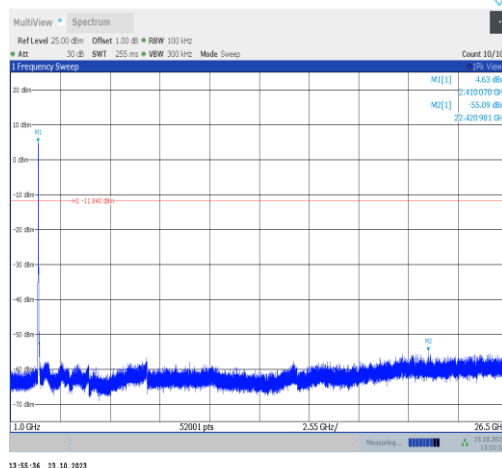
11g-Ant9-2412-1000~26500-PASS
