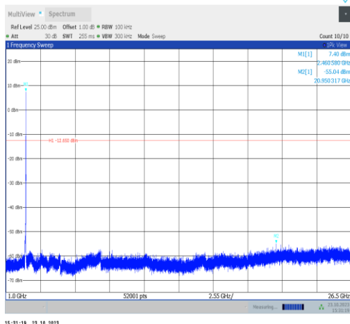
11n20SISO-Ant9-2462-1000~26500-PASS
