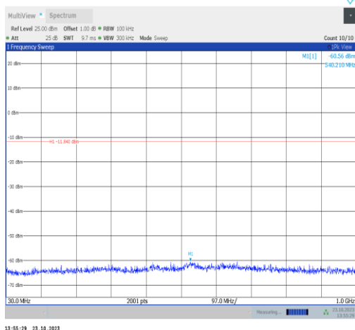
11g-Ant9-2412-30~1000-PASS
