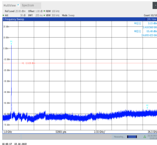
11n20SISO-Ant9-2412-1000~26500-PASS
