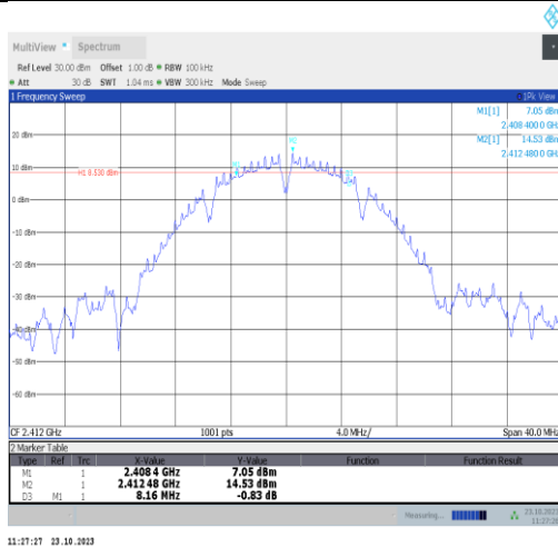
11b-Ant9-2412-PASS
