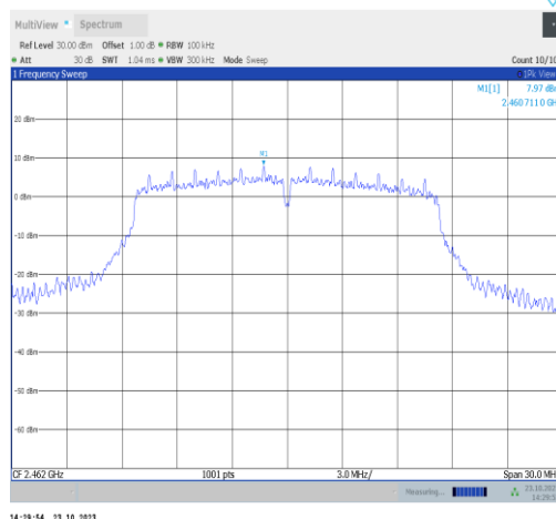
11g-Ant9-2462-0~Reference-PASS
