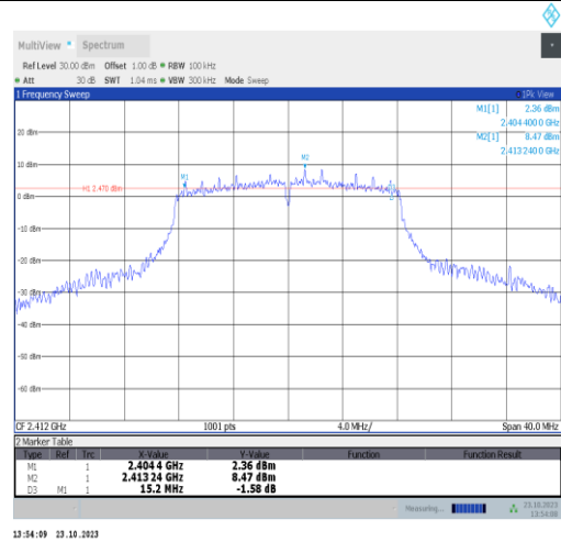
11g-Ant9-2412-PASS
