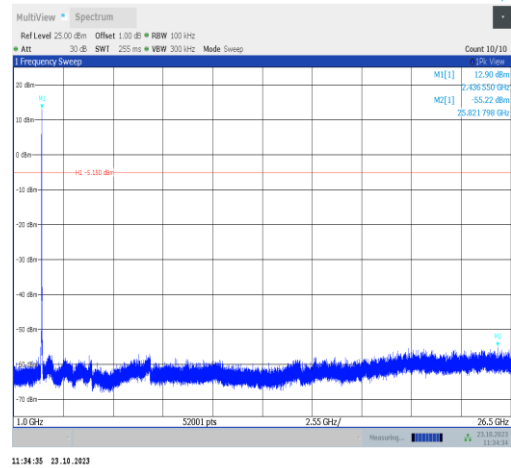
11b-Ant9-2437-1000~26500-PASS
