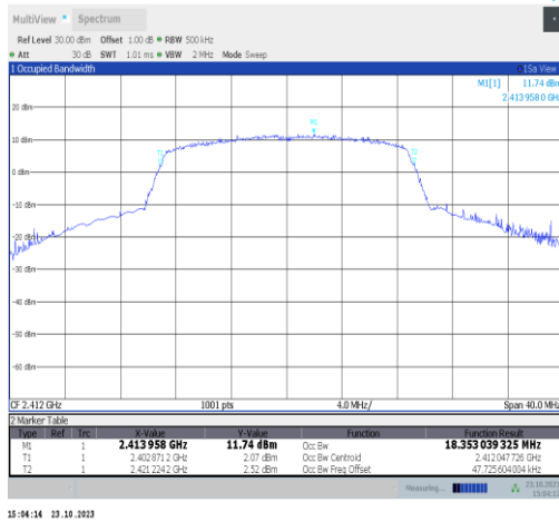
11n20SISO-Ant9-2412
