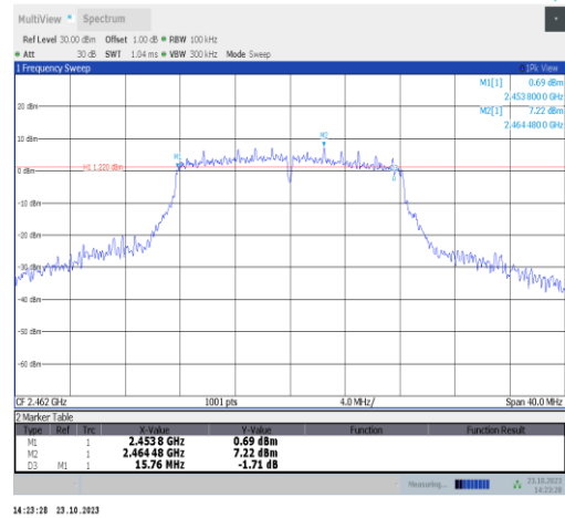
11g-Ant9-2462-PASS
