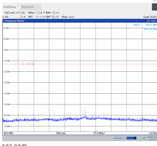
11n20SISO-Ant9-2437-30~1000-PASS
