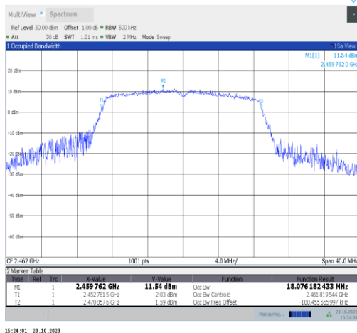
11n20SISO-Ant9-2462
