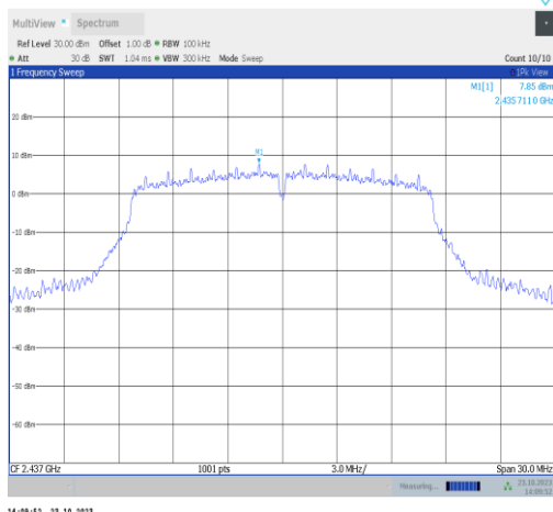
11g-Ant9-2437-0~Reference-PASS
