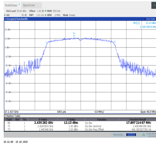
11n20SISO-Ant9-2437
