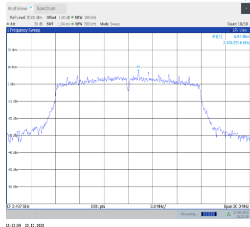
11n20SISO-Ant9-2437-0~Reference-PASS
