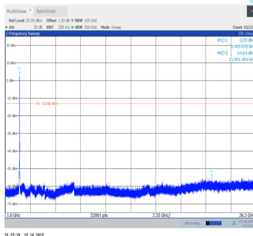
11n20SISO-Ant9-2437-1000~26500-PASS
