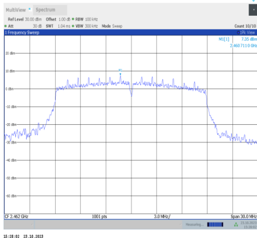
11n20SISO-Ant9-2462-0~Reference-PASS
