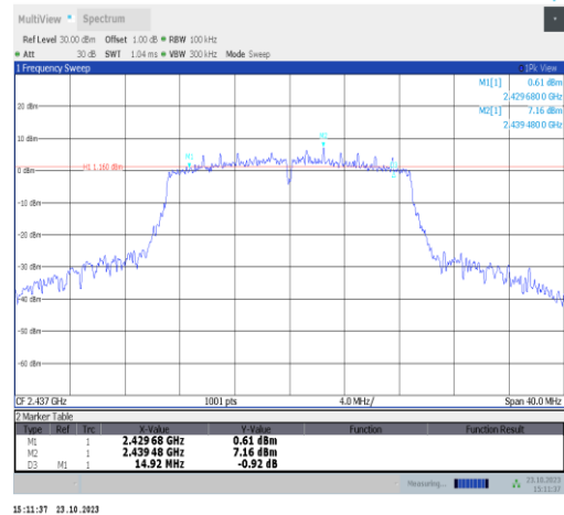
11n20ISO-Ant9-2437-PASS
