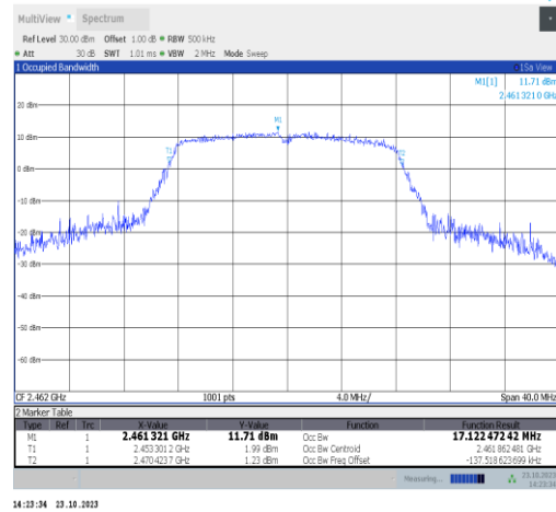
11g-Ant9-2462
