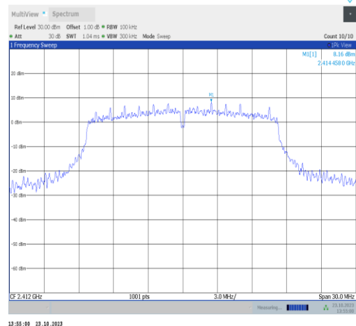
11g-Ant9-2412-0~Reference-PASS
