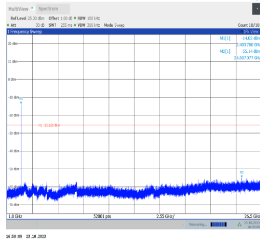
BLE_2M-Ant9-2404-1000~26500-PASS
