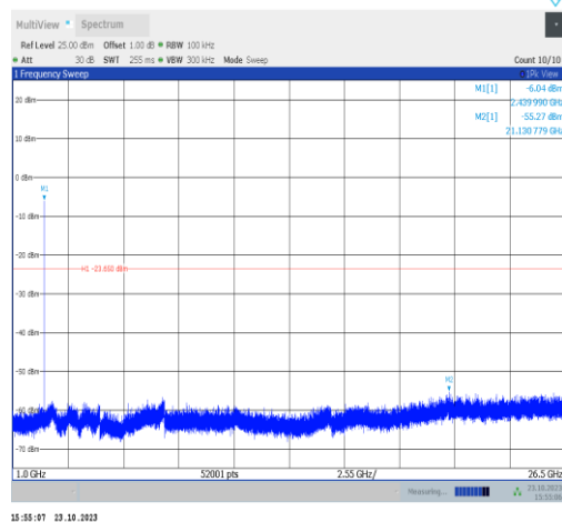
BLE_1M-Ant9-2440-1000~26500-PASS
