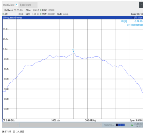
BLE_2M-Ant9-2440-0~Reference-PASS
