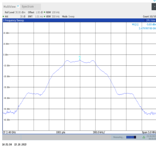
BLE_1M-Ant9-2480-0~Reference-PASS
