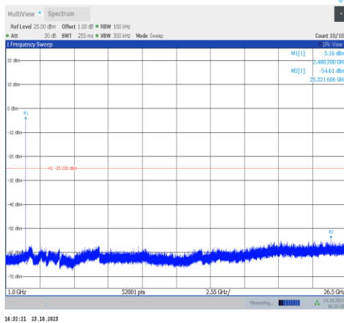
BLE_1M-Ant9-2480-1000~26500-PASS
