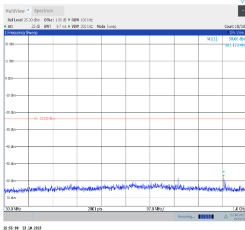
BLE_1M-Ant9-2440-30~1000-PASS
