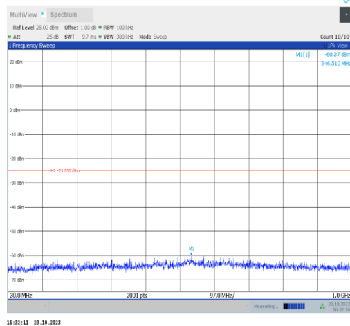
BLE_1M-Ant9-2480-30~1000-PASS
