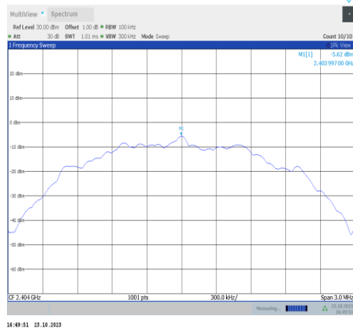
BLE_2M-Ant9-2404-0~Reference-PASS
