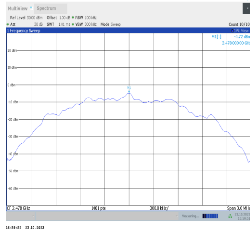
BLE_2M-Ant9-2478-0~Reference-PASS
