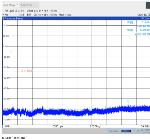
BLE_2M-Ant9-2440-1000~26500-PASS
