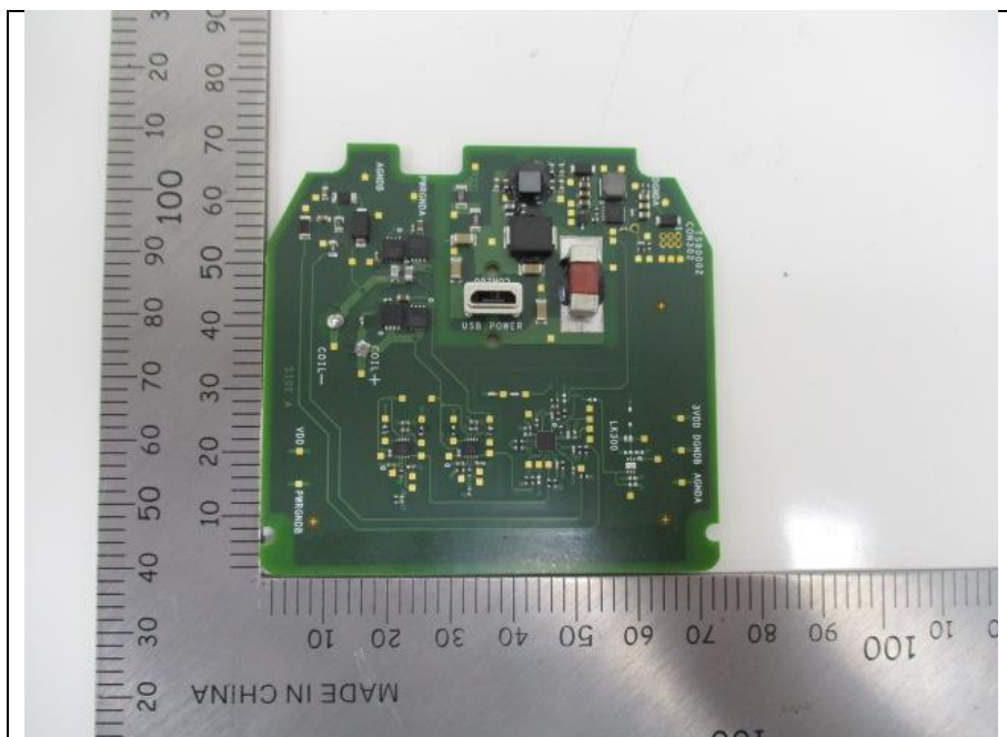
Main Board front side 2
