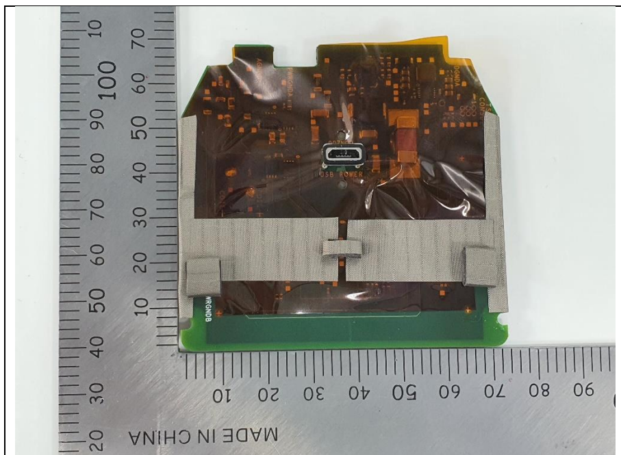
Main Board front side 1
