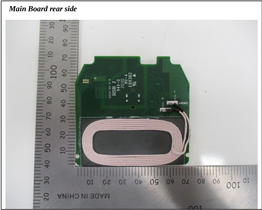
Main Board rear side 2
