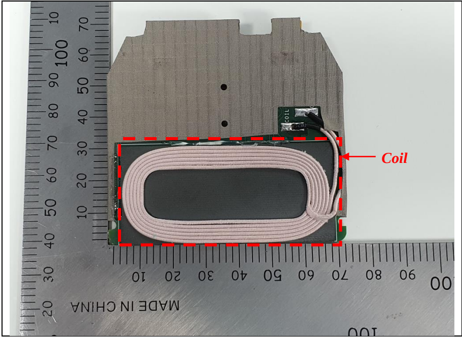
Main Board rear side 1
