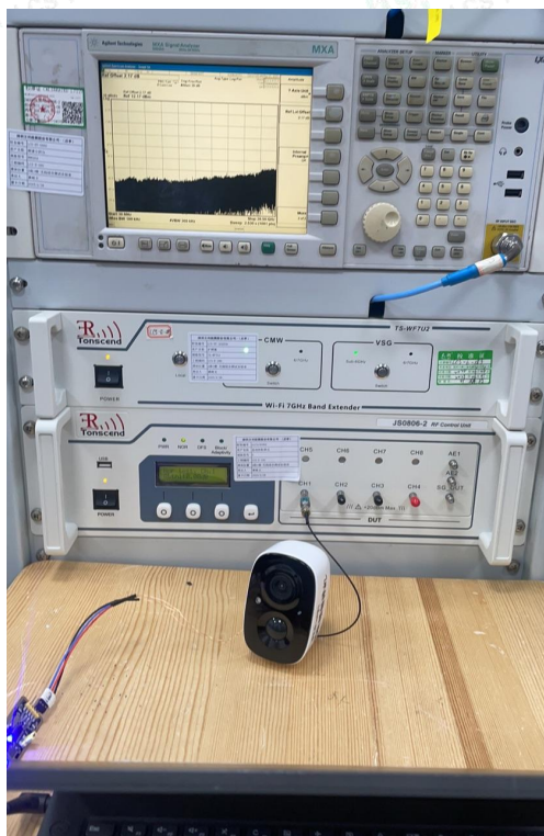
Fig. 3 Conducted Measurement
