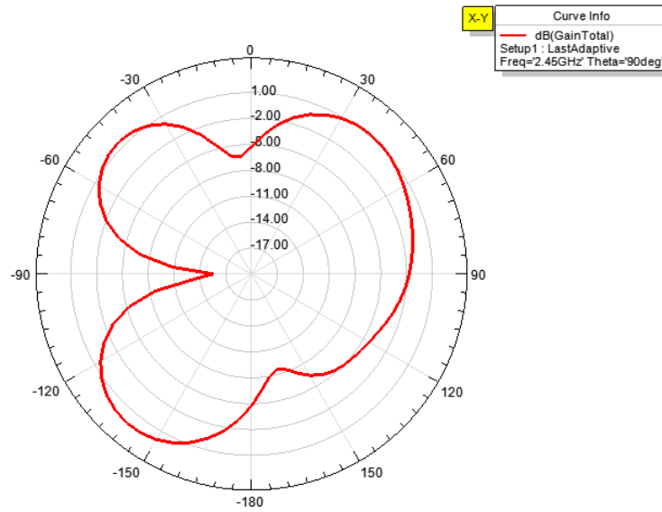
Radiation Pattern 2
