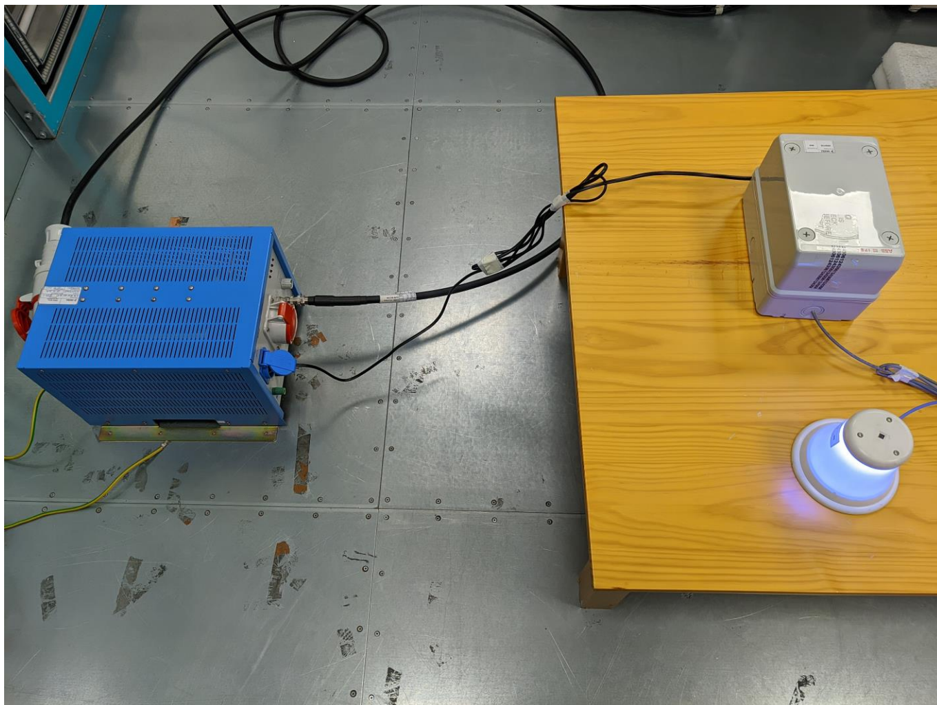
Conducted Emissions
