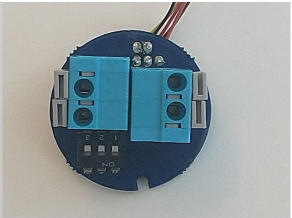
4 329452 PWB top
