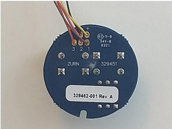
3 329452 PWB bottom
