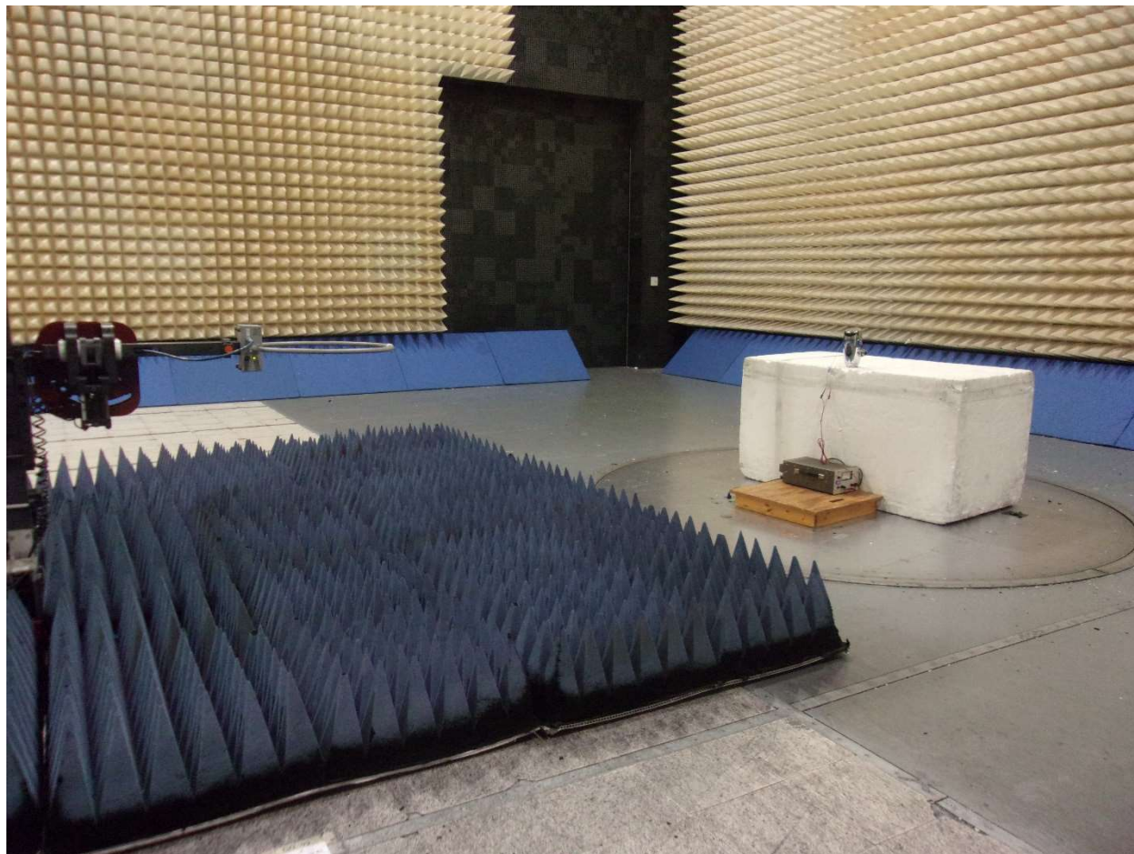
Radiated spurious emissions, 10kHz – 30MHz
